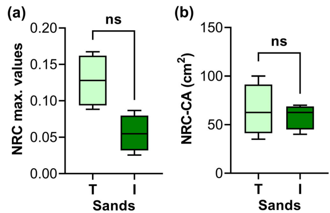
FIGURE 5 Impact of Amorpha fruticosa invasion and combined treatment (mowing and grazing) on the number of realized species combinations (NRC) (a) and characteristic areas (CAs) (b); CA represents the spatial scale at which the NRC reaches its maximum value. I, invaded and untreated vegetation type; T, invaded with combined treatment (mowed and grazed) vegetation type. Significance levels: ns, nonsignificant. Two-tailed paired t -test ( n = 4 ).
