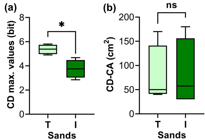
FIGURE 2 Impact of the Amorpha fruticosa invasion and combined nature treatment (mowing and grazing) on compositional diversity (CD) (a) and characteristic areas (CAs) (b) is examined; CA represents the spatial scale at which CD reaches its maximum value. I, invaded and untreated vegetation type; T, invaded with combined treatment (mowed and grazed) vegetation type. Significance levels: * p < 0.05 ; ns, nonsignificant. Two-tailed paired t -test ( n = 4 ).
