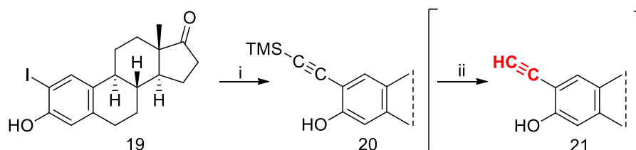
Scheme 4. Reagents and conditions: (i) 0.1 equiv. of Pd(PPh 3 ) 4 , 0.1 equiv. of CuI, 6 equiv. of Et 3 N, 2 equiv. of TMS-C≡CH, THF, MW, 50 °C, 20 min; (ii) 1 equiv. tetrabutylammonium fluoride (TBAF), toluene, 5 min.
