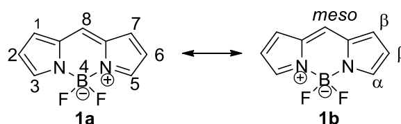
Figure 1. The core structure of 4,4-difluoro-4-bora-3a,4a-diaza-s-indacenes (BODIPY) dyes.
