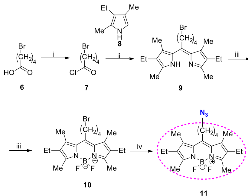
Scheme 2. Reagents and conditions: (i) 1.5 equiv. oxalyl chloride, \text{CH}_2\text{Cl}_2 , catalytic amount of N,N -dimethylformamide (DMF), rt, 2.5h; (ii) 2.5 equiv. of 8 , \text{CH}_2\text{Cl}_2 , reflux, 4h; (iii) 20 equiv. \text{Et}_3\text{N} , reflux, 30 min, 20 equiv. \text{BF}_3 \cdot \text{OEt}_2 , reflux, 4 h; (iv) 1 equiv. of \text{NaN}_3 , DMSO, catalytic amount of AcOH.
