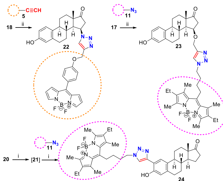
Scheme 5. Reagents and conditions: (i) \text{CuI} (0.05 equiv.), \text{Ph}_3\text{P} (0.1 equiv.), \text{DIPEA} (3 equiv.), 1 equiv. \text{TBAF} , toluene, reflux, 2 h; (ii) \text{CuI} (0.05 equiv.), \text{Ph}_3\text{P} (0.1 equiv.), \text{DIPEA} (3 equiv.), toluene, reflux, 2 h.
