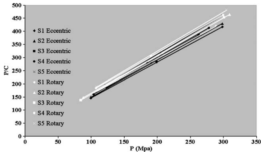
Fig. 4. Kawakita plot calculated with the out-of-the-die method
