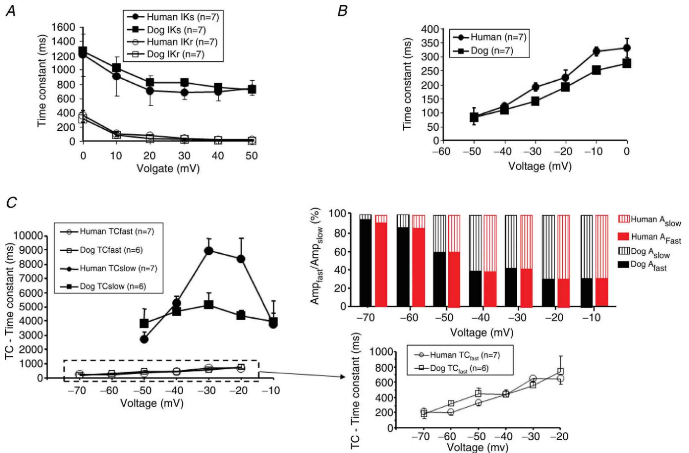
Figure 4. The voltage dependence of the activation and deactivation kinetics of human and canine I_{Kr} and I_{Ks} A, voltage dependence of activation kinetics. I_{Kr} and I_{Ks} were activated by test pulses with durations from 10 to 5000 ms, to test potentials ranging from 0 to 50 mV; then the cells were clamped back to -40 mV. The amplitudes of tail currents as a function of the duration of the depolarization were well fitted by single exponentials. B, the voltage dependence of I_{Ks} deactivation kinetics was determined by activating I_{Ks} with 5000 ms test pulses to 50 mV from a holding potential of -40 mV. Then the cells were clamped back for 2 s to potentials ranging from -50 to 0 mV (pulse frequency 0.1 Hz) and the deactivation time course of the tail current was fitted by a single exponential function. C, the voltage dependence of I_{Kr} deactivation kinetics was determined by activating I_{Kr} with 1000 ms test pulses to 30 mV from a holding potential of -40 mV. Then the cells were clamped for 16 s to potentials ranging from -70 to 0 mV (pulse frequency 0.05 Hz) and the deactivation time course of the tail current was fitted by a double exponential function. The left panel shows the voltage dependence of slow and fast time constants. An expanded version of the results for voltage dependence of the fast time constants is provided in the right bottom panel. The right top panel shows the relative amplitudes of the fast and slow components at different voltages in dog (black) and human (red) ventricular myocytes.
