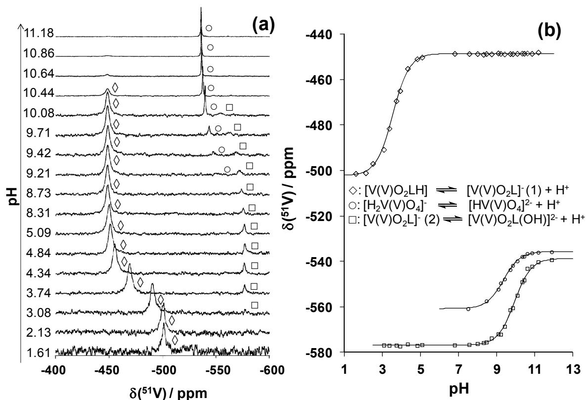
Fig. 7. ^{51}\text{V} NMR spectra recorded for the V(V) – STSC system at various pH values (a) and chemical shifts of the various groups of species plotted against the pH (b). \diamond: [\text{V}(\text{V})\text{O}_2\text{LH}] \rightleftharpoons [\text{V}(\text{V})\text{O}_2\text{L}]^- (1) + \text{H}^+ ; \circ: [\text{H}_2\text{V}(\text{V})\text{O}_4]^- \rightleftharpoons [\text{HV}(\text{V})\text{O}_4]^{2-} + \text{H}^+ ; \square: [\text{V}(\text{V})\text{O}_2\text{L}]^- (2) \rightleftharpoons [\text{V}(\text{V})\text{O}_2\text{L}(\text{OH})]^{2-} + \text{H}^+ . \{c_{\text{V}(\text{V})} = 1.8 \text{ mM}; \text{V}(\text{V}):\text{L} = 1:1.1; T = 25.0^\circ\text{C}, I = 0.10 \text{ M (KCl) in } 30\% \text{ (v/v) DMSO, } 60\% \text{ (v/v) H}_2\text{O, } 10\% \text{ (v/v) D}_2\text{O.}\}
