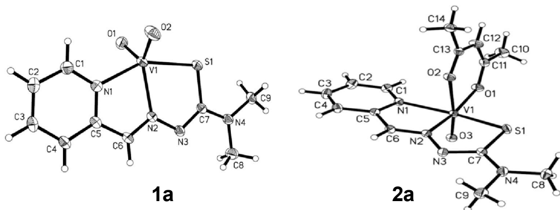
Fig. 5. ORTEP view of [\text{V(V)}\text{O}_2(\text{L})] complex of PTSC ( 1a ) and [\text{V(IV)}\text{O}(\text{L})(\text{acac})] complex of PTSC ( 2a ) with thermal ellipsoids at 50% probability level. Selected bond distances and angles are summarized in Table S2.
