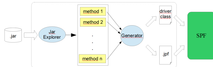
Figure 3: Architecture of the runtime environment
