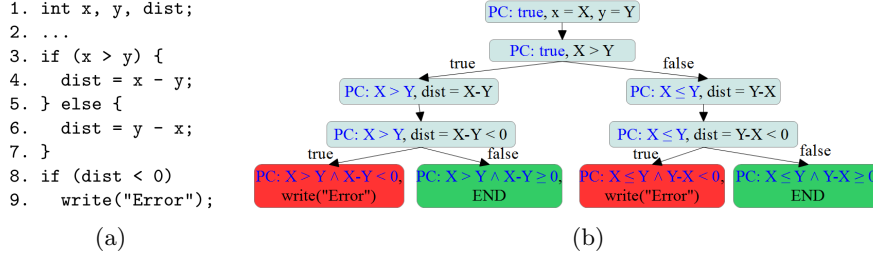
Figure 1: (a) Sample code that determines the distance of two integers on the number line (b) Symbolic execution tree of the sample code handling variable x and y symbolically
