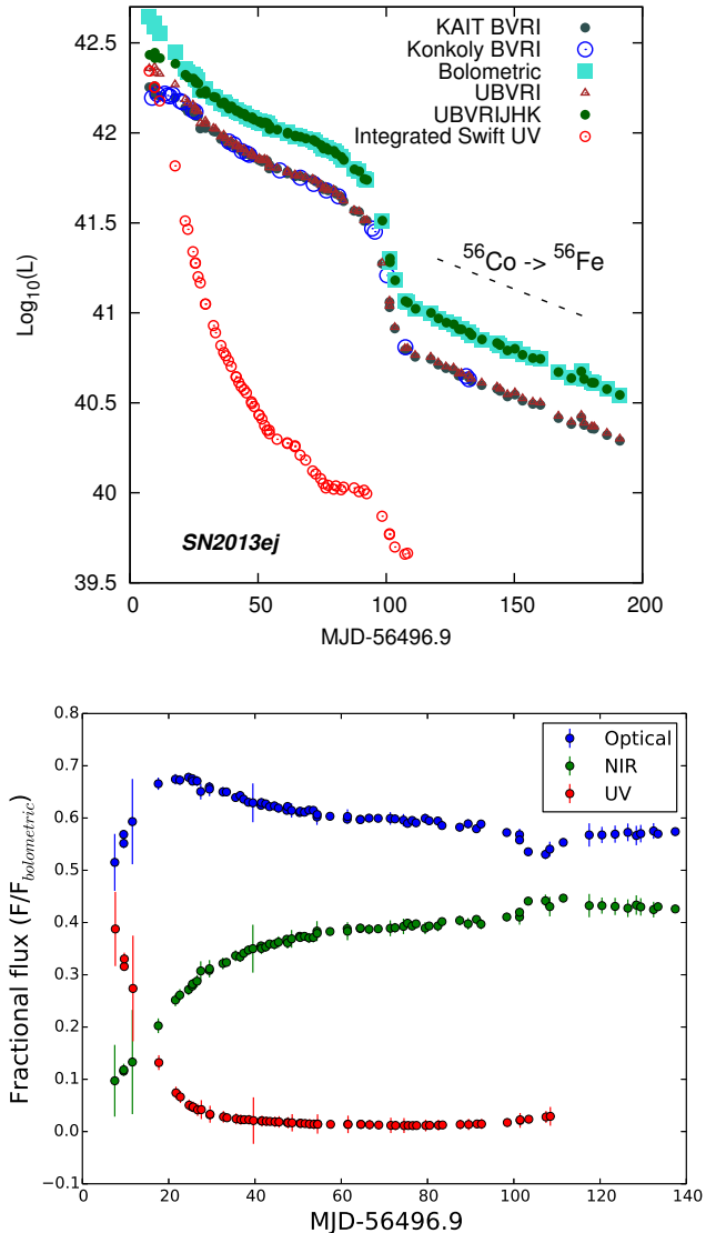
FIG. 11.— Top Panel: Integrated BVRI , UBVRJHK , and bolometric light curves of SN 2013ej. UBVRJHK and UBVRJHK shown here are derived using Swift u , KAIT BVRI , RATIR JH , and estimated flux from the K band. The bolometric light curve includes an additional contribution from UV flux below \sim 3200 \text{ \AA} before +30d. Beyond +30d, UBVRJHK closely resembles the bolometric light curve in the plateau. Bottom Panel: UV, optical, and near-IR fractional flux. The UV covers flux below the U band, the near-IR (NIR) covers flux above the I band, while optical covers in between ( UBVRJHK ). The UV fraction is shown curtailed at the calculated end of plateau, because of the marginal contribution and possible contamination from red tails (see text).
