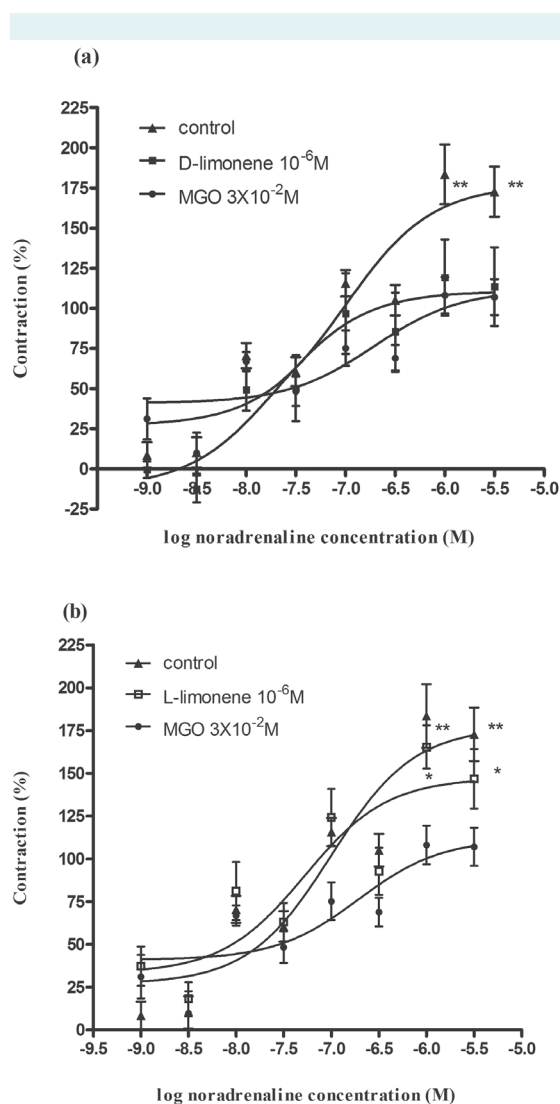
FIGURE 5. The effect of d-limonene ( 10^{-6} M) (A) and l-limonene ( 10^{-6} M) (B) on the noradrenaline-evoked (control) uterine contractions in the presence of methylglyoxal ( 3 \times 10^{-2} M) and \beta -adrenoreceptor antagonist propranolol ( 10^{-5} M) (Dunnett's multiple comparison test, P=0.043 ).
