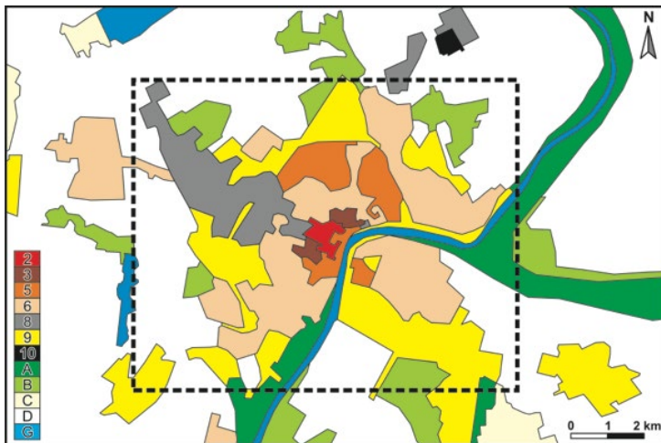
Fig. 1. The obtained LCZ map in Szeged (LCZ 2 – compact mid-rise, LCZ 3 – compact low-rise, LCZ 5 – open mid-rise, LCZ 6 – open low-rise, LCZ 8 – large low-rise and LCZ 9 – sparsely built, LCZ A – dense trees, LCZ B – scattered trees, LCZ C – bush, scrub, LCZ D – low plants, LCZ G – water) and the study area (broken line)
