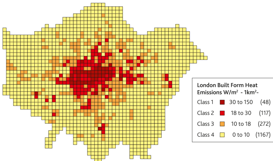
■ Figure 5. Annual average heat emission from buildings (1x1 km) in London (2005) (Hamilton et al., 2009)
