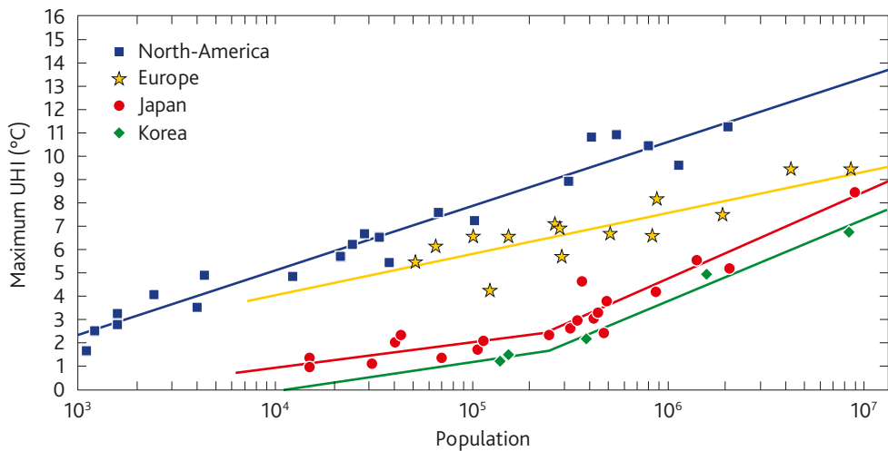
Figure 17. Relation between maximum UHI intensity and population for North-American, European, Japan and Korean settlements (Oke, 1973; Park, 1987)
