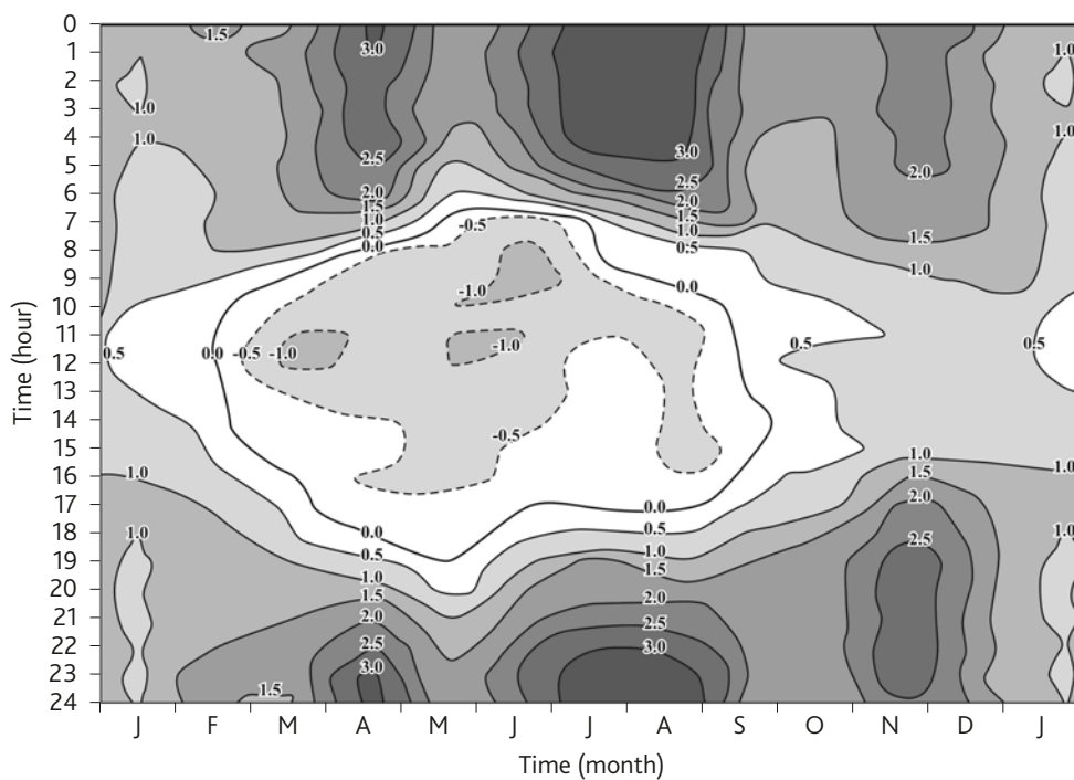
■ Figure 16. Annual and diurnal variation of UHI intensity
