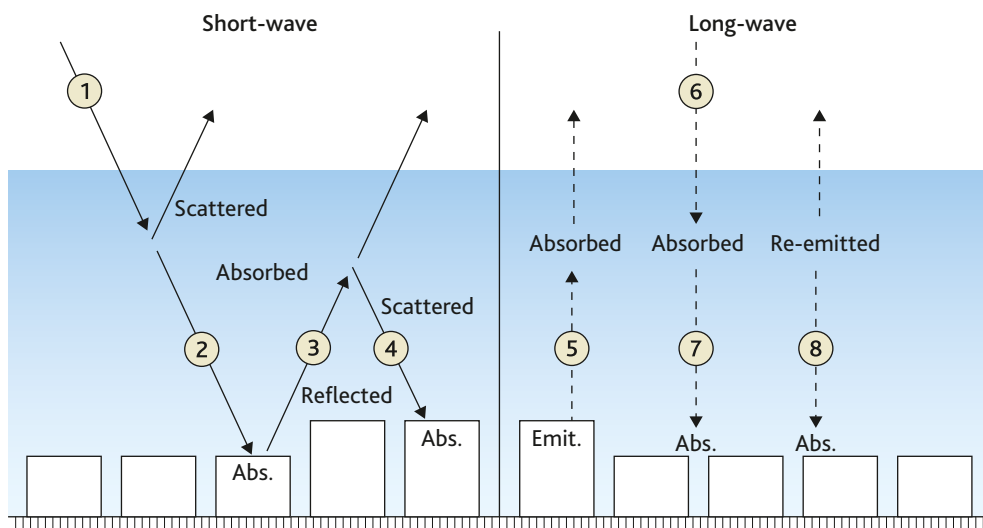
Figure 8. Schematic depiction of radiative exchanges in a polluted urban boundary layer (Oke, 1982)
