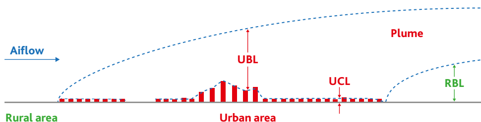
■ Figure 7. Schematic representation of the urban atmosphere with its two layers (the slope of the UBL is between 1:100 and 1:200 in reality) (Oke 1976)
