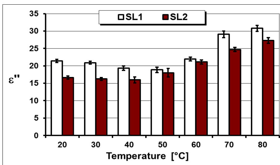
Fig. 1. Change of dielectric loss factor with temperature
