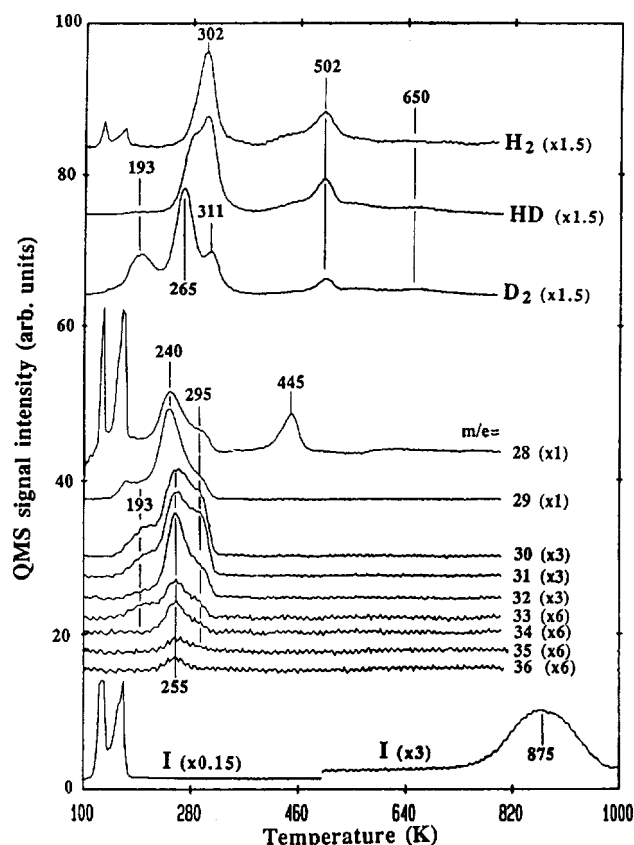
Figure 11. TPD spectra taken after coadsorbing 0.47 ML D and multilayer C_2H_3I on Pt(111) at 100 K. Heating rate was 6 K/s.
