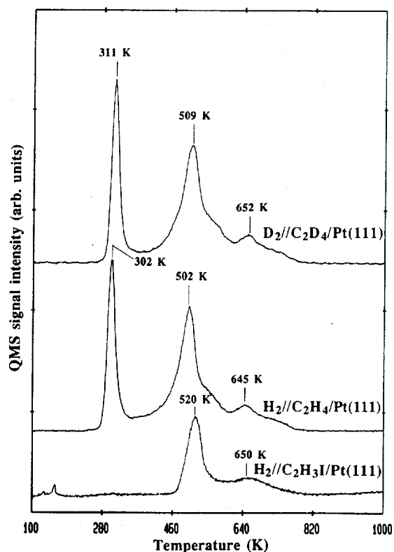
Figure 4. TPD spectra of dihydrogen for saturated monolayer C_2H_3I , C_2H_4 , and C_2D_4 . The exposure temperature was 100 K, and the heating rate was 6 K/s.
