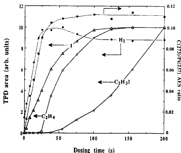
Figure 3. Exposure time dependence of TPD areas, from Figures 1 and 2, for H_2 , C_2H_4 , I, and C_2H_3I , and of the C(273)/Pt(237) AES ratio.
