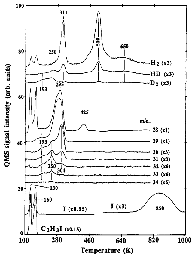
Figure 10. TPD spectra taken after coadsorbing 0.18 ML D and multilayer C_2H_3I on Pt(111) at 100 K. Heating rate was 6 K/s.
