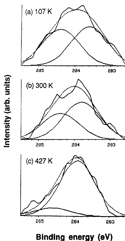
Figure 6. C(1s) XPS core level spectra for a multilayer dose of C_2H_3I on Pt(111) at 70 K, then warmed briefly to (a) 107 K, (b) 300 K, and (c) 427 K. All spectra were taken after recooling to below 100 K. The broad, somewhat noisy spectra are the experimental data, while the smooth curves are synthesized fits using Gaussian profiles.
