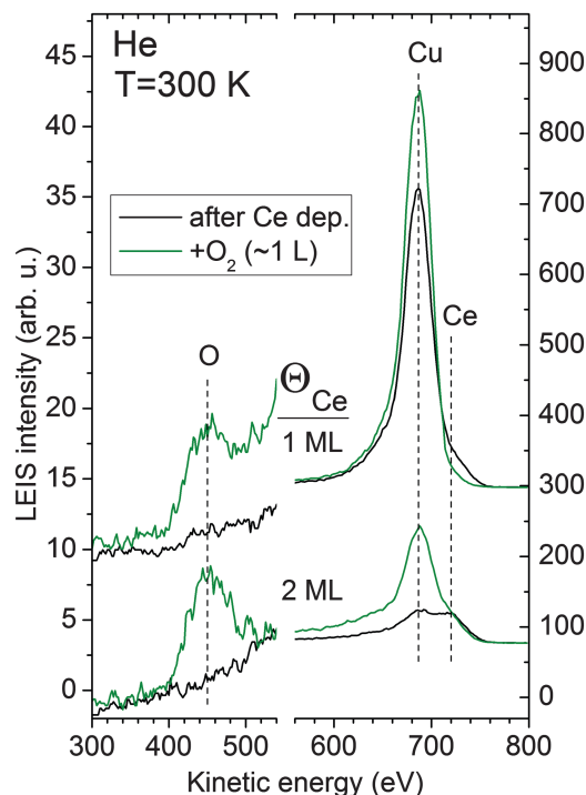
Fig. 4 LEIS spectra obtained with He after the deposition of Ce on Cu(111) at 300 K and after subsequent adsorption of \text{O}_2 ( \sim 1 \text{ L} ) at 300 K.
