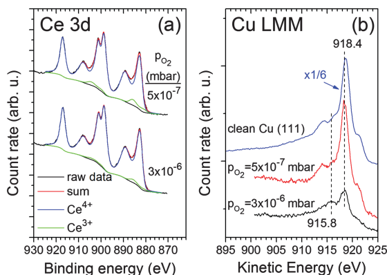
Fig. 7 The Ce 3d XPS region (a) and the Cu LMM Auger region (b) after the deposition of 16 ML of CeO 2 on Cu(111) at varying O 2 pressures. In (b) the Cu LMM region for the clean Cu(111) surface is also presented.
