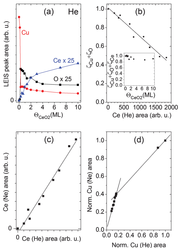
Fig. 5 Deposition of Ce on Cu(111) at T = 523 K in an O_2 background of 3 \times 10^{-6} mbar, (a) areas of LEIS peaks obtained with He as a function of CeO_2 coverage, (b) the fraction of the surface covered by Cu and O, calculated using the relative sensitivity factor S_O = 0.0191 , displayed as a function of the Ce (He) area. Inset: \zeta_{Cu} + \zeta_O + \zeta_{Ce} as a function of CeO_2 coverage, (c) the Ce area obtained with neon as a function of Ce area obtained with helium, (d) the normalized Cu area obtained with neon as a function of the normalized Cu area obtained with helium. For (b), (c) and (d) linear fits are also presented.
