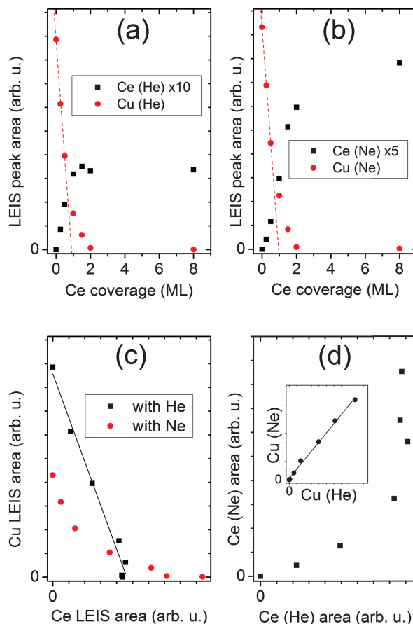
Fig. 3 The change of Ce and Cu LEIS peak area obtained with He (a) and Ne (b) during the deposition of Ce on Cu(111) at 300 K. Linear fits on the first three Cu areas (up to a cerium coverage of 0.5 ML) are presented as dashed lines for both (a) and (b). In (c) the Cu LEIS area is shown as a function of the Ce area with both He and Ne. For the data points obtained with He a linear fit is also displayed. In (d) the Ce (Ne) area obtained in the same experiment is plotted against the Ce (He) area, while in the inset the Cu (Ne) area is shown as a function of the Cu (He) area. For the latter a linear fit is also presented.
