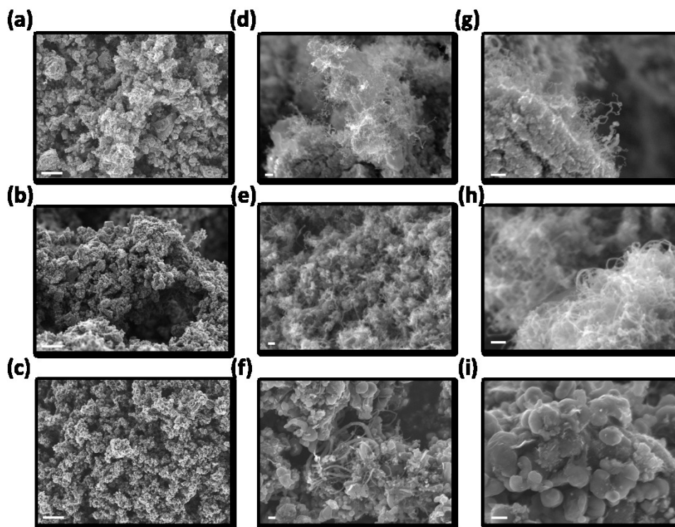
Figure 1 SEM images of porous structure of carbon growth on nickel mesoporous layer at (a, d, g) 400°C, (b, e, h) 600°C, (c, f, i) 800°C, the scale bar of (a-c) and (d-i) are 10 \mu\text{m} and 200 nm respectively.
