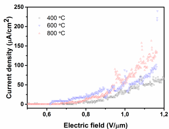
Figure 6 Field emission of carbon/Raney nickel composites.
