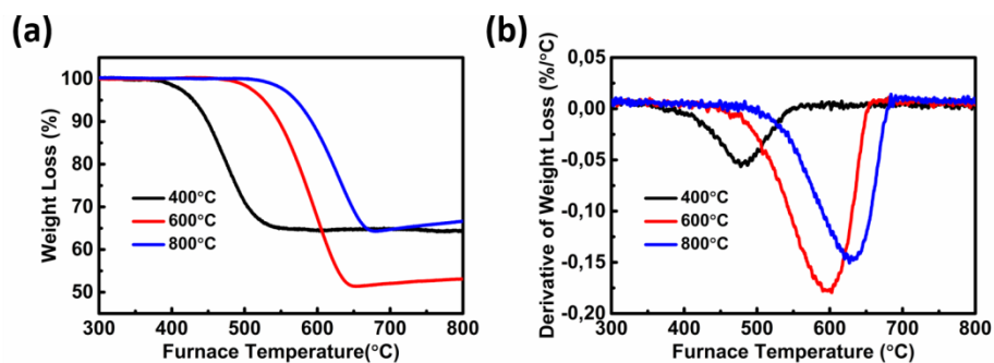
Figure 4 (a) Weight loss and (b) differential thermal gravimetric curves for different nanostructured Ni-carbon composites.
