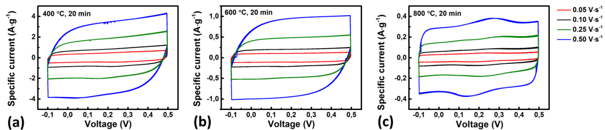
Figure 5 Cyclic voltammetry curves with different charge/discharge rates of carbon grown on nickel mesoporous layer after (a) 400°C, (b) 600°C, and (c) 800°C growth process.
