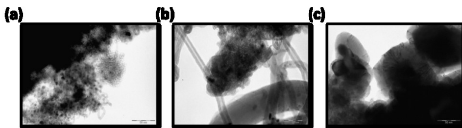
Figure 2 TEM images of carbon structure on nickel mesoporous layer after (a) 400°C, (b) 600°C, and (c) 800°C growth.
