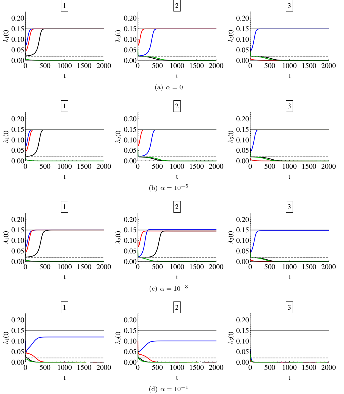
Figure 7: Solutions of system (T_1) – (T_3) with HIV dynamics for different travel volumes. The three regions are considered to be symmetric in every parameter value, we applied the parameter set given in Section 7 so that \mathcal{R}_c^i < \mathcal{R}_H^i < 1 is satisfied for i = 1, 2, 3 . We use the reducible connection network depicted in Figure 3 (a), where the connectivity potential parameters c^{12} , c^{21} , c^{23} are equal to one in all model classes. Solid and dashed gray lines correspond to steady state solutions in the regions in the absence of traveling.
