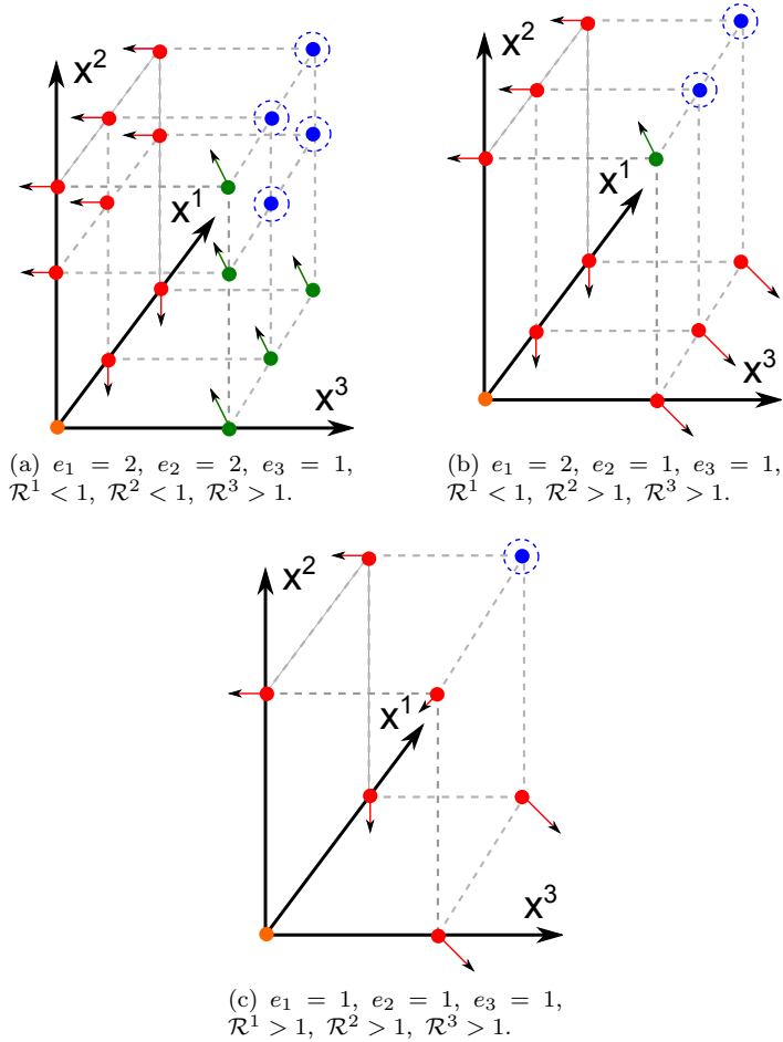
Figure 1: We illustrate the behavior of steady states in the system of three regions connected to each other by a complete mobility network, for three different cases in the values of local reproduction numbers. Dots on the schematic diagrams depict infected components of equilibria of the disconnected system, and e_i denotes the number of positive fixed points in region i , i = 1, 2, 3 . Mobility has no impact on the disease free equilibrium (orange dot). Componentwise positive steady states (blue dots) are preserved in the system with traveling, as they continuously depend on the mobility parameter \alpha . A boundary endemic equilibrium moves out from the nonnegative octant with the introduction of traveling if the equilibrium has a component corresponding to a region, which is disease free in the absence of traveling and has local reproduction number ( \mathcal{R} ) greater than one (red dot). Other boundary steady states move into the interior of the nonnegative octant (green dots).
