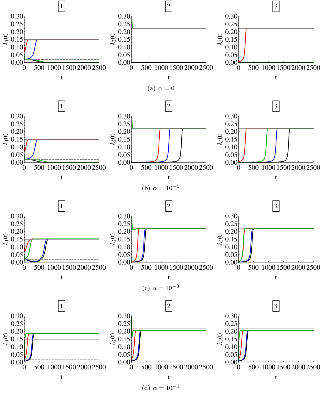
Figure 10: Solutions of system (T_1) – (T_3) with HIV dynamics for different travel volumes. The three regions are considered to be symmetric in every parameter value but the local reproduction numbers, we applied the parameter set given in Section 7 with \beta_1^i = 0.85 and \beta_2^i = \beta_3^i = 1 so that \mathcal{R}_c^1 < \mathcal{R}_H^1 < 1 and \mathcal{R}_H^2, \mathcal{R}_H^3 > 1 are satisfied. We use the complete connection network depicted in Figure 3 (c), where the connectivity potential parameters c^{ij} , i, j \in \{1, 2, 3\} , i \neq j , are equal to one in all model classes. Solid and dashed gray lines correspond to steady state solutions in the regions in the absence of traveling.
