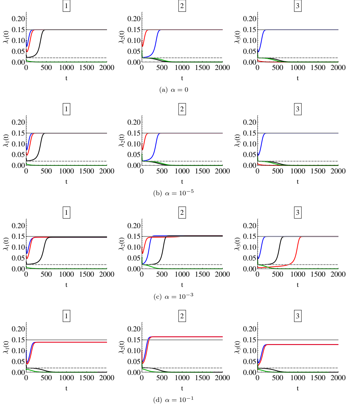
Figure 6: Solutions of system (T_1) – (T_3) with HIV dynamics for different travel volumes. The three regions are considered to be symmetric in every parameter value, we applied the parameter set given in Section 7 so that \mathcal{R}_c^i < \mathcal{R}_H^i < 1 is satisfied for i = 1, 2, 3 . We use the irreducible connection network depicted in Figure 3 (b), where the connectivity potential parameters c^{12} , c^{21} , c^{23} , c^{31} are equal to one in all model classes. Solid and dashed gray lines correspond to steady state solutions in the regions in the absence of traveling.
