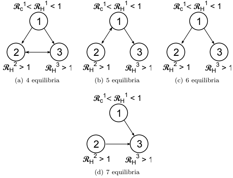
Figure 4: Examples of the travel network for three regions with \mathcal{R}_c^1 < \mathcal{R}_H^1 < 1 and \mathcal{R}_H^2, \mathcal{R}_H^3 > 1 .
