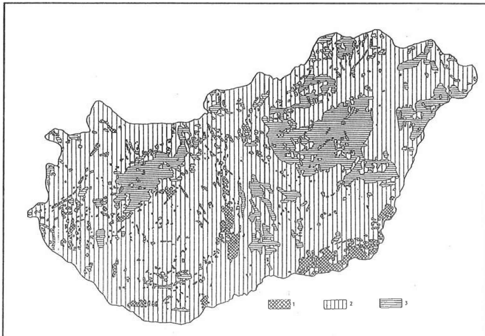
Figure 2 Superimposed map of the limiting natural factors.
