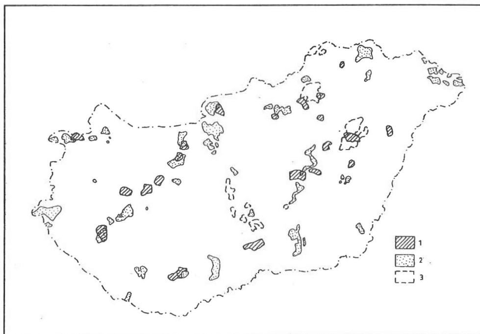
Figure 6 Critical environmental areas in Hungary 1 - critical environmental areas; 2 - landscape protection areas; 3 - natural parks.
