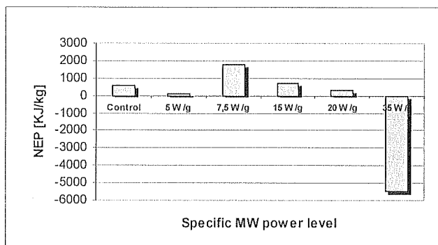
Fig. 6.: The net energy product by anaerobic fermentation
