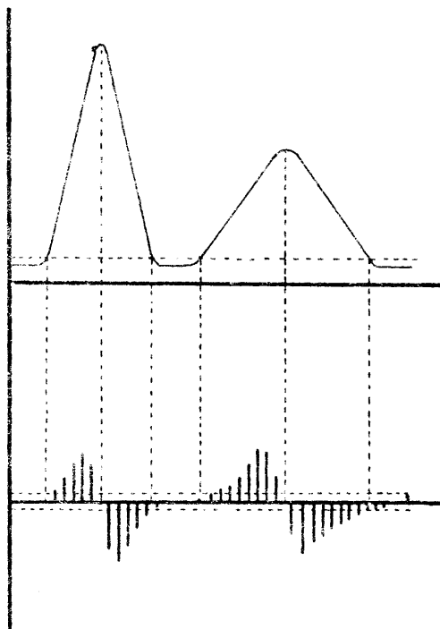
Figure 6.: Peak recording using the changing tendencies.
