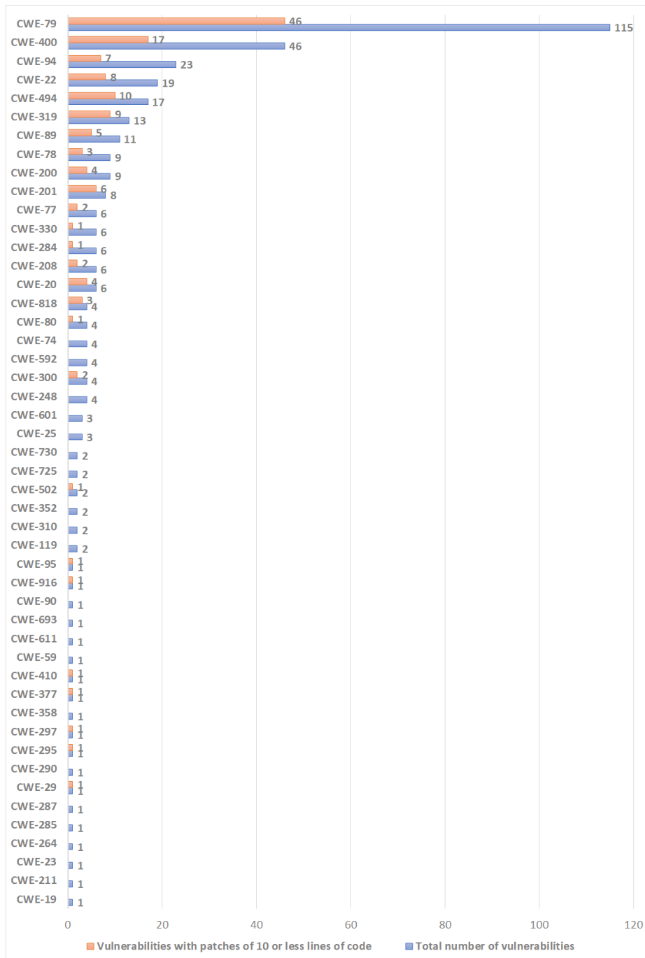
Fig. 3. Number of total vulnerabilities and mitigation patches with 10 lines or less, grouped by CWE categories
