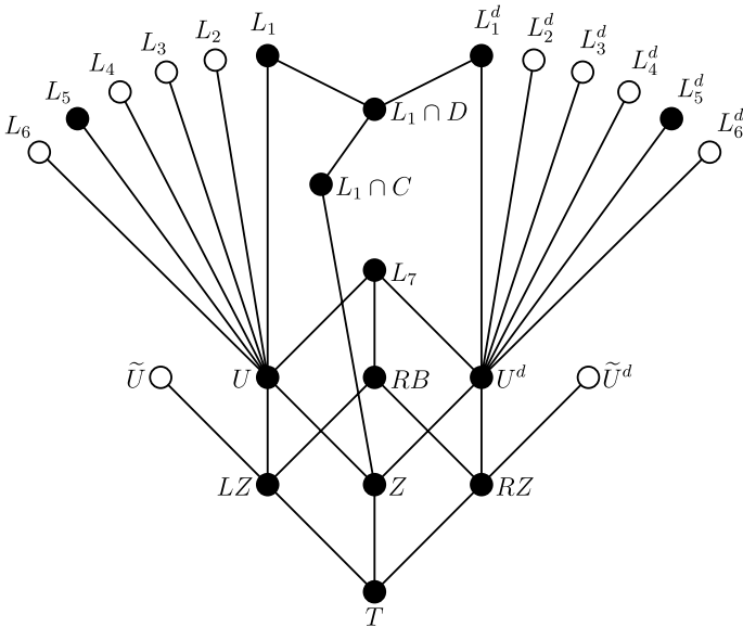
Fig. 1 The semilattice of lazy groupoid varieties
