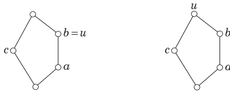
FIGURE 3. The elements a, b and c (with an example u proving (a, c, b), (b, a, c) \in T ) in case (N_5)
