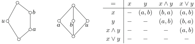
FIGURE 2. Counterexamples showing that these equations do not belong to \mathcal{E}
