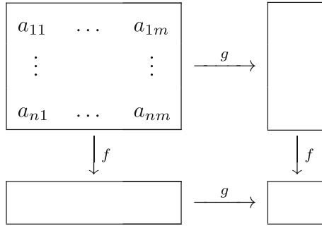
FIGURE 1. Commutation of f and g
