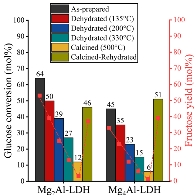
Fig. 7 Catalytic performances of the as-prepared and treated Mg 2 Al-LDH and Mg 4 Al-LDH. Reaction conditions: glucose (100 mg), ethanol (14 mL), catalyst (100 mg), T = 80\text{ }^{\circ}\text{C} , t = 2\text{ h} . Squares indicate fructose yield. (The dash-dotted lines are just a guide to the eye.)
