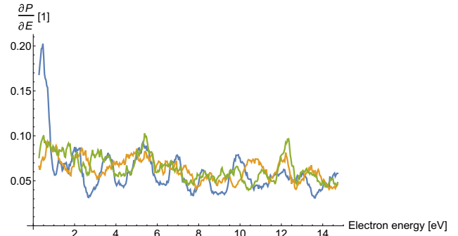
Fig. 3. Energy spectrum of the continuum electron. The blue, orange and green lines are for I = 10^{12} , 2.5 \times 10^{13} and 8.1 \times 10^{13} W cm ^{-2} , respectively.
