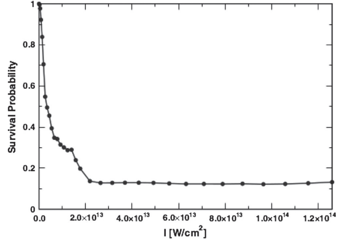
Fig. 1. Stabilization of the potassium atom in a superatomic field: survival probability vs. laser intensity for a 800 nm, 65 fs laser pulse. For details, see reference [30].
