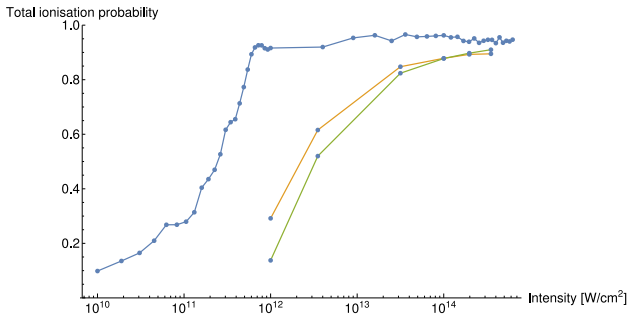
Fig. 2. Total ionisation probabilities as a function of the laser intensity. \lambda = 800 nm, \tau = 120 fs. The blue line corresponds to the ab initio calculations, the orange and the green to CTMC simulations with the model potentials (30) and (31), respectively.
