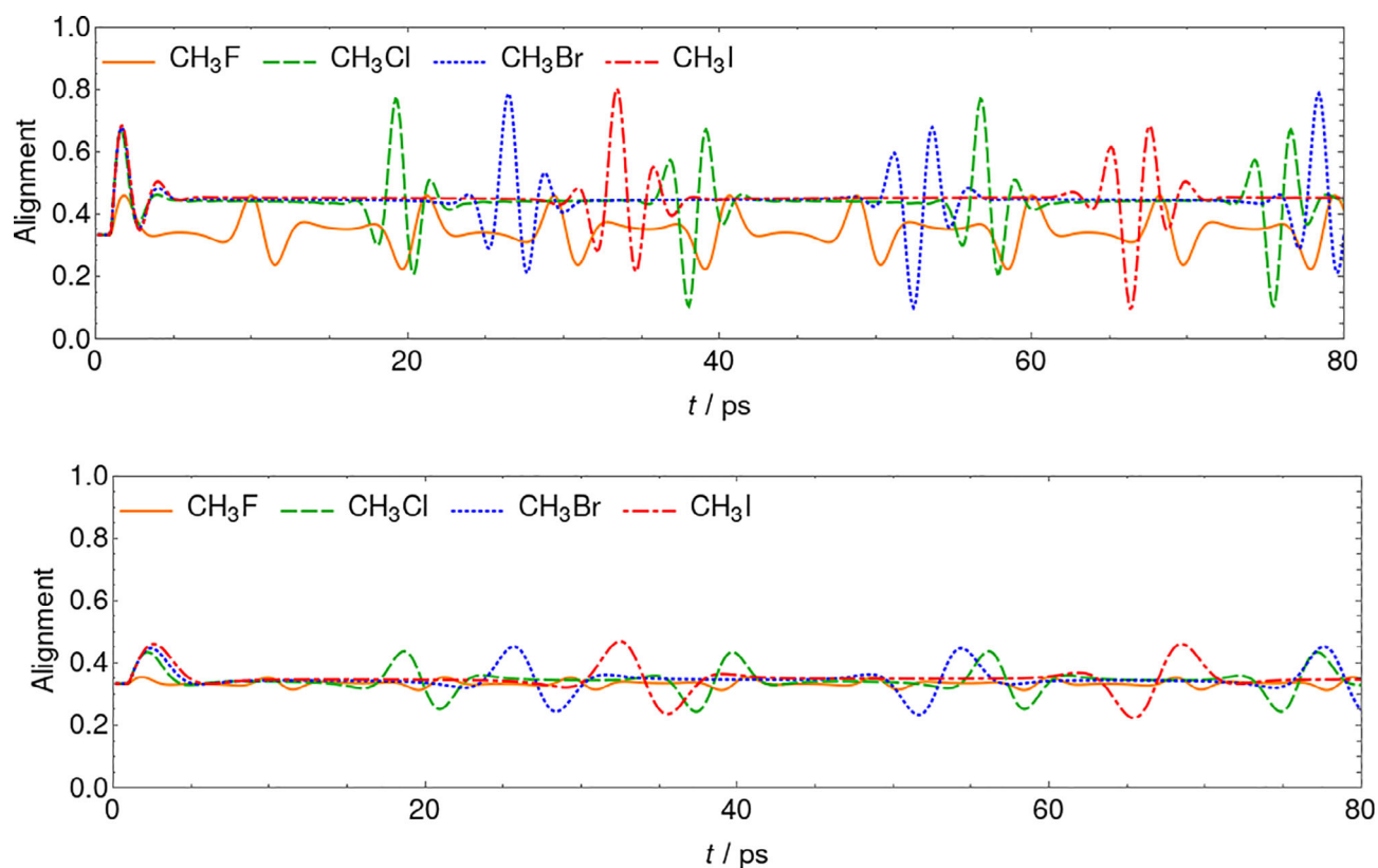
FIGURE 1 Comparison of the laser-induced rotational alignment of the \text{CH}_3\text{X} molecules for a medium- and a high-intensity optical pulse. The pulse parameters chosen are as follows: T/\text{K} = 5 , \lambda/\text{nm} = 800 , I/\text{TW cm}^{-2} = 30 (upper panel) and 5 (lower panel), \text{FWHM}/\text{fs} = 100 , and the pulse position is 1 ps
