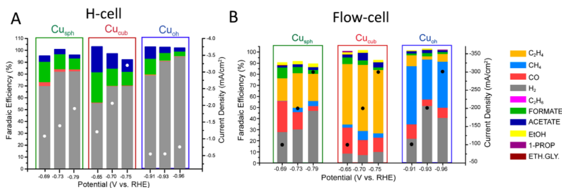
Fig. 3 Selectivity of the same Cu nanocatalysts in an H-cell using a CO 2 -saturated 0.1 M KHCO 3 electrolyte (A) and in a gas-fed microfluidic flow cell with a flowing 1 M KOH electrolyte (B). Reproduced from ref. 17. Copyright 2020 ACS.
