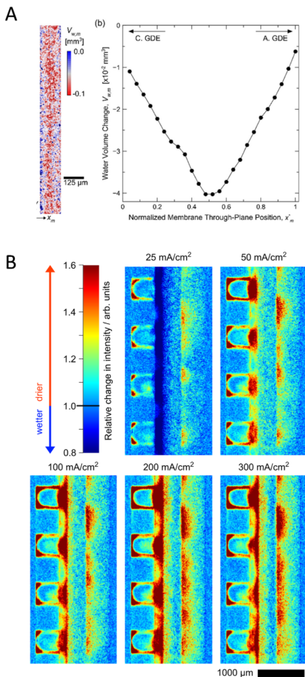
Fig. 11 Operando visualisation and quantification of water management in \text{CO}_2 electrolyzers. (A) Quantification of liquid water content in a MEA by neutron radiography. Processed image highlighting the water volume change in the CEM. Water-volume change across the membrane is plotted on the graph. Reproduced from ref. 91. Copyright 2020 ACS. (B) Relative change in the water-content of a zero-gap \text{CO}_2 electrolyzer during operation. Reproduced from ref. 100. Copyright the Authors, published by Springer Nature.
