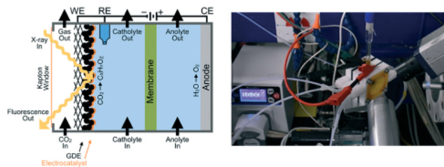
Fig. 5 Schematic illustration and photograph of a microfluidic operando XAS cell allowing for fluorescence measurements. Reproduced from ref. 115. Copyright 2020 RSC.
