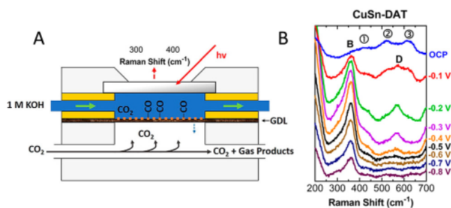
Fig. 7 (A) Schematic and photograph of a Raman spectroelectrochemical flow cell hosting a gas diffusion electrode. The cell mimics the conditions of a microfluidic CO 2 electrolyzer. (B) Operando SERS of a CuSn electrode during CO 2 RR measured in the cell. Peak B is assigned to the frustrated rotational mode of adsorbed CO on Cu. Peaks D and 1, 2, 3 are SnO 2 - and Cu 2 O-related bands. Reproduced from ref. 125. Copyright 2019 ACS.
