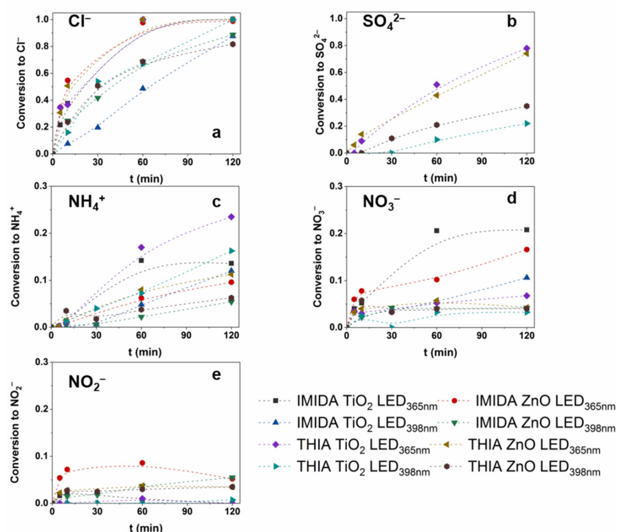
Figure 7. The conversion of organic Cl-, S-, and N-content of IMIDA and THIA to \text{Cl}^- (a), \text{SO}_4^{2-} (b), \text{NH}_4^+ (c), \text{NO}_3^- (d) and \text{NO}_2^- (e).
