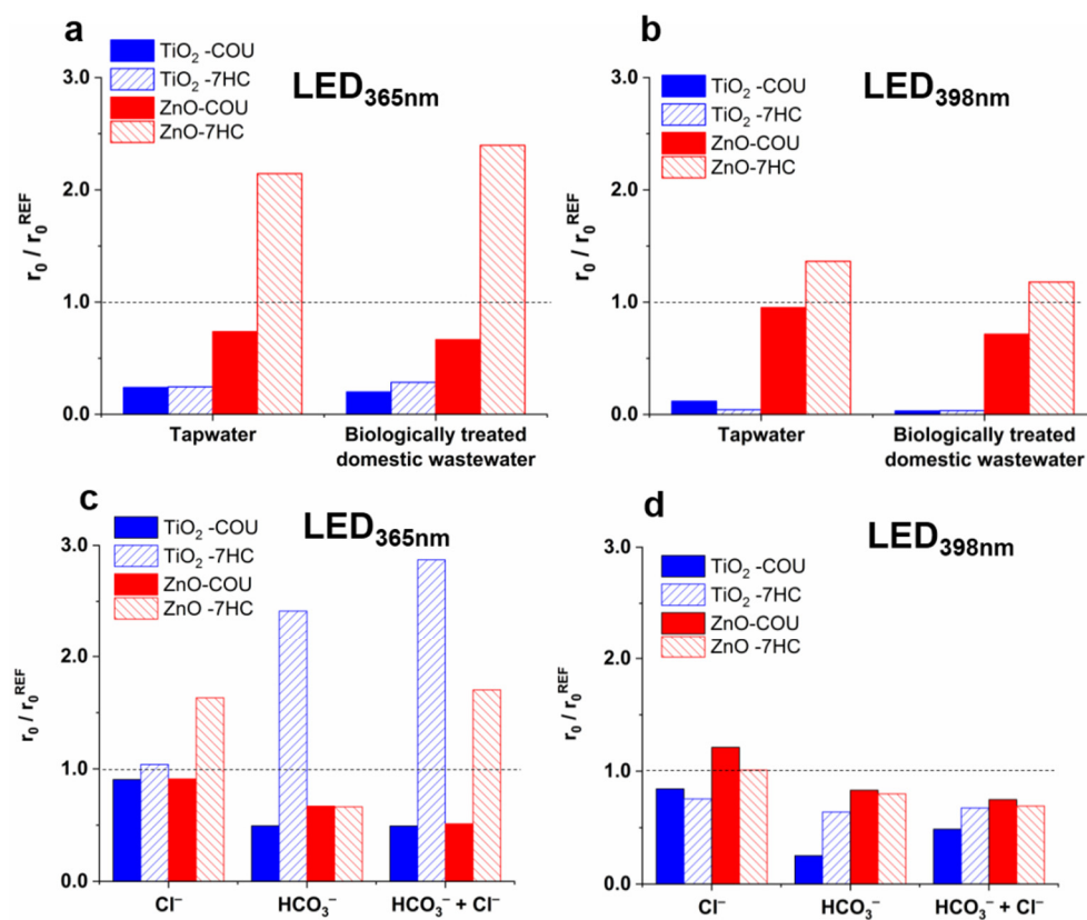
Figure 3. Effect of matrices (a,b), Cl^- (120 mg dm -3 ), and HCO_3^- (525 mg dm -3 ) (c,d) on the relative transformation rate of COU and formation rate of 7-HC.
