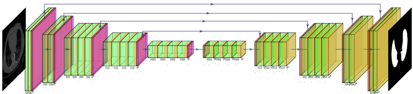
Figure 5. VGG-SegNet architecture.
