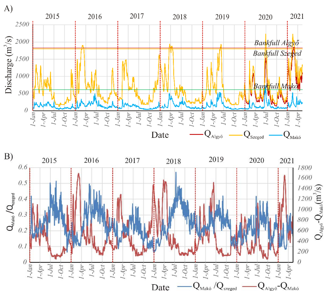
Figure 3. (A) Daily discharge values at the three gauging stations and (B) the discharge ratio ( Q_{Makó}/Q_{Szeged} ) and difference ( Q_{Algyő} - Q_{Makó} ) at the gauging stations of the Tisza (Algyő and Szeged) and the Maros (Makó) in the studied period (January 2015–May 2021).
