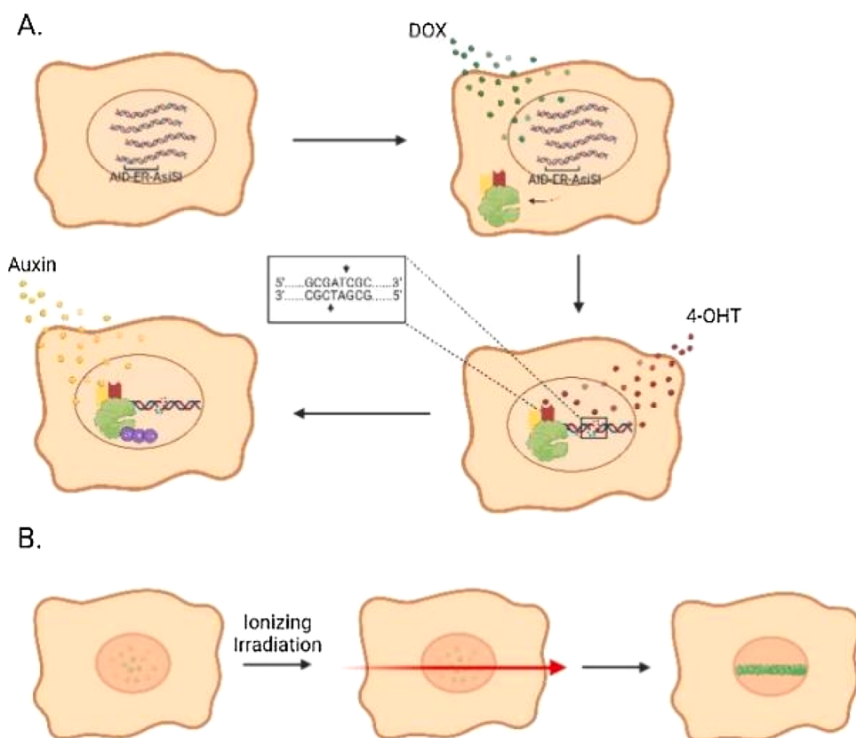
Fig. 1. A: Schematic representation of DlvA (DSB Induction via AsiSI) cell line engineered in the laboratory of Gaëlle Legube, stably expressing the AID-ER-AsiSI. Upon doxycycline (DOX) addition, the protein is expressed and sequesters in the cytoplasm. 4-OHT addition induces the translocation of the AID-ER-AsiSI into the nucleus, where it sequence-specifically cleaves the DNA. Auxin treatment leads to the ubiquitylation and degradation of the protein. B: DNA damage response upon ionizing radiation recruits GFP-tagged DNA repair proteins at the damaged foci in the nucleus.
