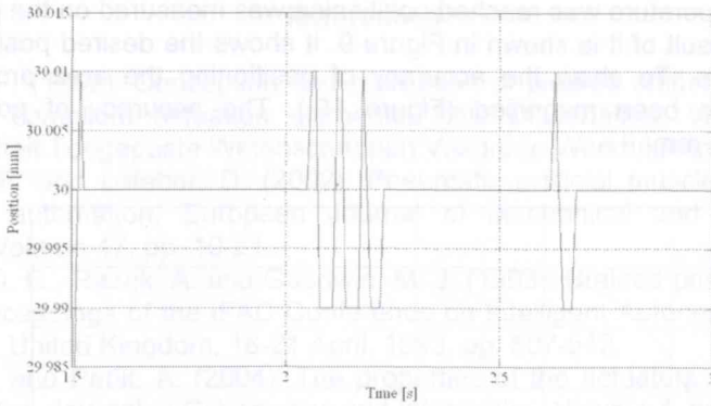
Figure 6. Position as a function of time (enlarged)
