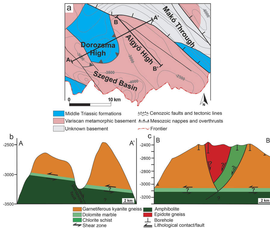
Fig. 13. Theoretical geologic sections of the studied area: (a) generalized pre-Cenozoic basement map of the studied area (modified after Haas et al., 2010); (b) cross-section across the DH and the northwestern part of AH along the line A-A'; (c) NW-SE profile of AH along the line B-B'. The Dorozsma Fault is after Tari et al. (1999)
