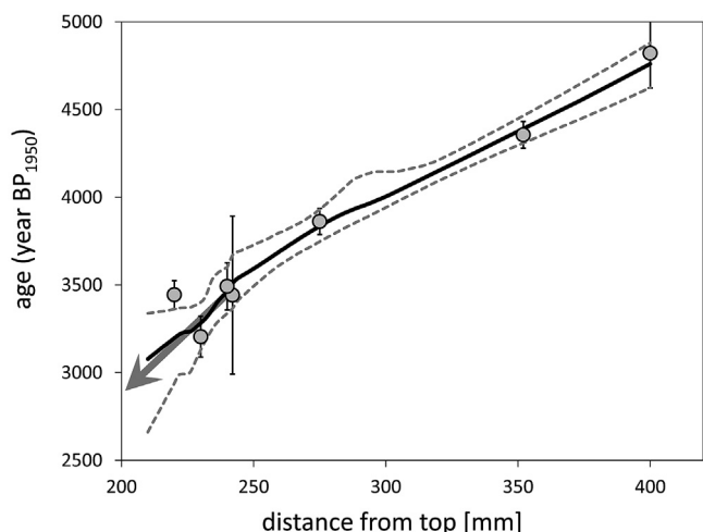
Fig. 2. An age-depth model established from the original U/Th data of Siklósy et al. (2009) using the StalAge algorithm (Scholz and Hoffmann, 2011). The grey arrow marks the direction to the origin.
