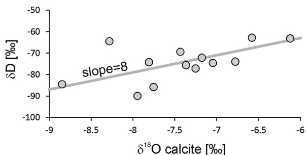
Fig. 7. Stable hydrogen isotope compositions (relative to V-SMOW) of inclusion-hosted water and oxygen isotope compositions of the host calcite (relative to V-PDB) at the inclusion sampling intervals of the Trió stalagmite. The grey line (arbitrarily placed within the sample points) marks slope = 8 characteristic for the Global Meteoric Water Line (Craig, 1961).
