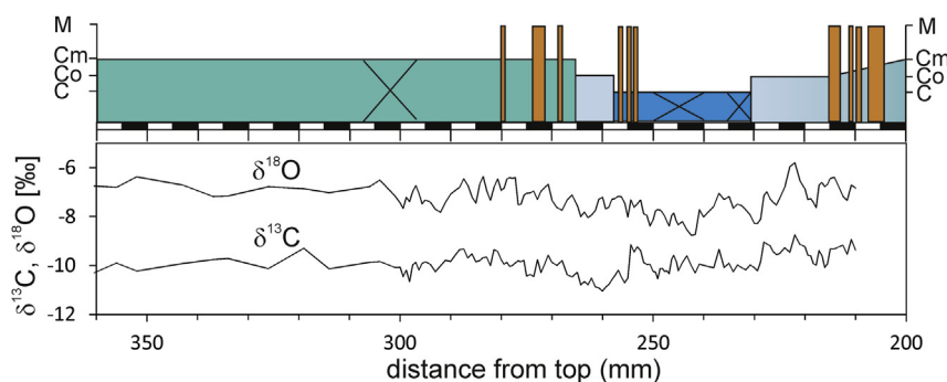
Fig. 6. Microstratigraphic log of the section between 200 and 360 mm from the top of Trió stalagmite along with stable C and O isotope compositions. Sections not covered with thin sections are marked by X. C: Dense columnar calcite (light blue). Co: porous columnar calcite (dark blue). Cm: Microcrystalline calcite, Ms: micrite/microsparite with high detrital content.
