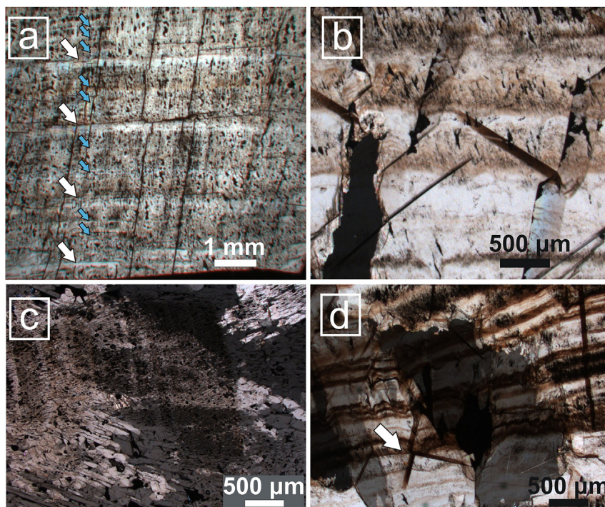
Fig. 4. Carbonate fabrics occurring in the Trió core. (a) Porous columnar fabric with two orders of lamination (sub-laminae connected to thin detrital layers are aligned by blue arrows, while the macroscopically visible compact laminae are aligned by white arrows). (b) Compact columnar fabric with low porosity. (c) Microcrystalline fabric with inter-fingering extinction boundaries and high porosity. (d) Erosion surface in the lowermost section of the compact columnar fabric aligned by white arrow, covered by a series of brown laminae of detrital origin.
