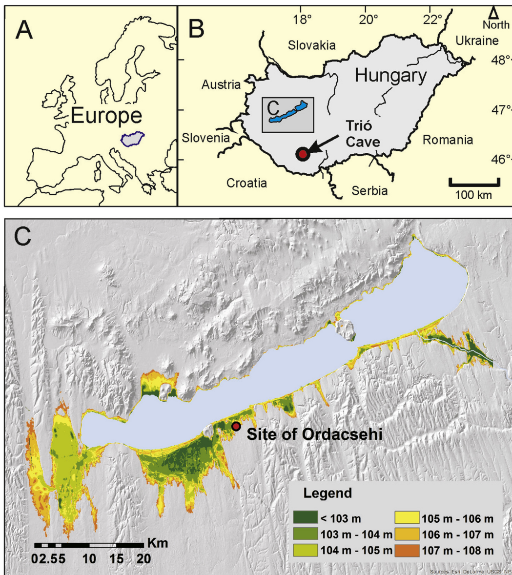
Fig. 1. Locations of the archaeological site of Ordacsehi-Bugaszeg (bivalve shells) and the Trió Cave (stalagmite). Potential lake water levels are shown in C as heights above sea level.
