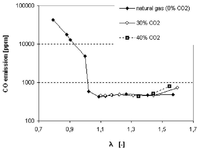
Figure 2. CO emission
