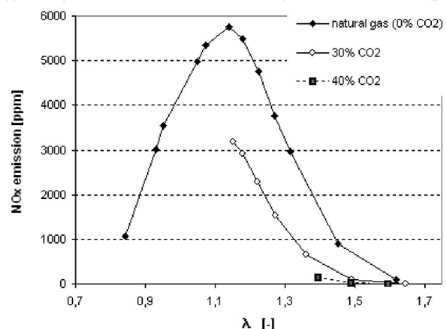
Figure 1. \text{NO}_x emission
