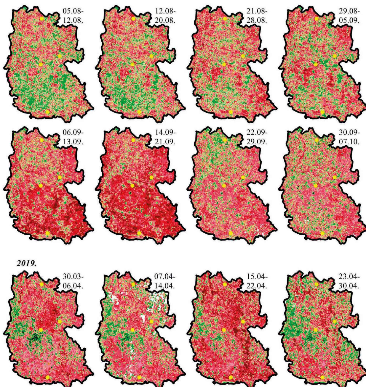
Figure 4.4. Spatial analysis of standardised NDDI in 2018-2019
