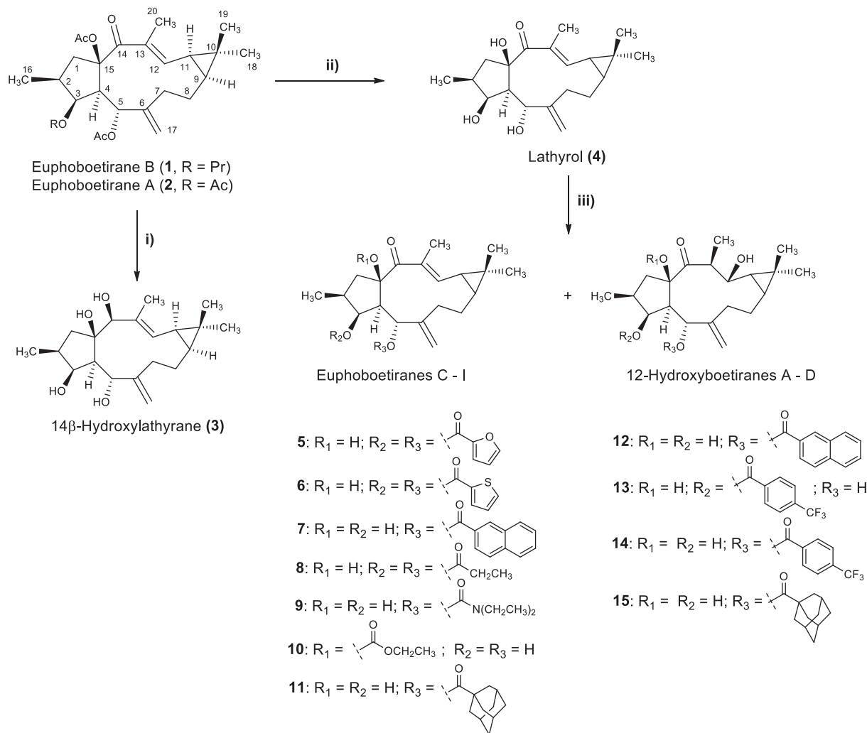
FIGURE 1 Chemical structures of lathyrane diterpenes ( 1 and 2 ) isolated from Euphorbia boetica aerial parts and preparation of 14β-hydroxylathyrane ( 3 ), lathyrane ( 4 ) and derivatives ( 5–15 ). Reagents and conditions: (i) LiAlH 4 , THF, 0°C, 1 h; (ii) KOH/MeOH (5%), room temperature, 3 h; (iii) acylating reagent, DMAP (cat.), TEA/CH 2 Cl 2 (1:1), room temperature or under reflux (60°C, nitrogen atmosphere), 2–18 h
