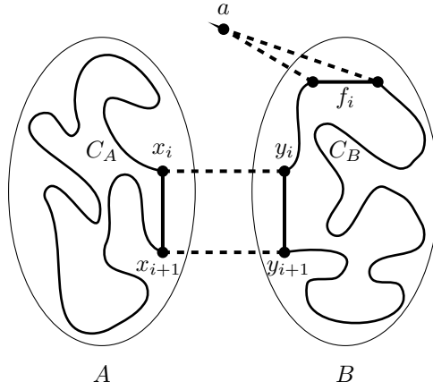
FIGURE 2.1.1. Transforming the problem of finding a Hamiltonian cycle on V(G') into finding two Hamiltonian cycles C_A and C_B on A and B respectively.
