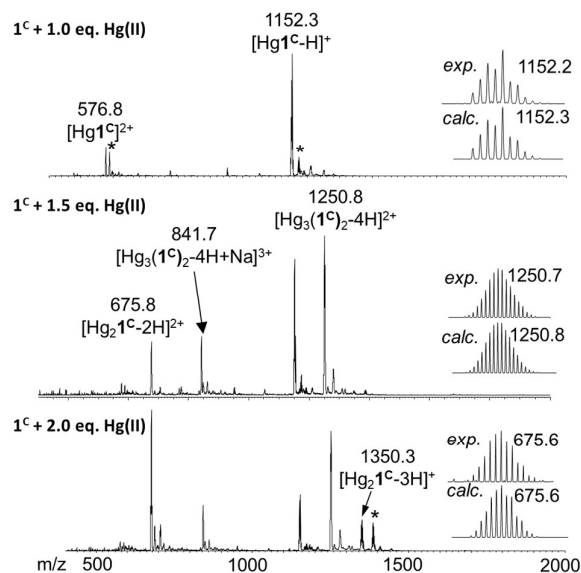
Figure 3. (+)ESI-MS spectra registered for 1^C with different equivalents of Hg(II) in ammonium acetate buffer (20 mM, pH = 6.9). The comparison of the experimental and calculated isotopic envelope of the detected species are also presented. Asterisks mark the sodium adduct of the corresponding species. The notation 1^C refers here to the neutral free peptide.
