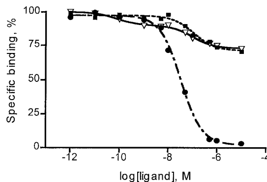
Fig. 3. The 480-AON induced change in the receptor density investigated by radioligand receptor binding assay. The concentration of [ ^3 H]prazosin was 1.5 nM and the concentration of the unlabeled ligand was varied between 10^{-5} and 10^{-12} M. The displacement curves demonstrate the lack of the \alpha_{1A} -AR subtypes in 480-AON-treated rat uteri. The WB4101 ( \alpha_{1A} -AR subtype-selective) binds to a single class of binding sites in the 480-AON-treated rat uterus membrane preparation, whereas it recognizes two binding sites in the nontreated rat uterus preparation; the high-affinity binding site is identical with the \alpha_{1A} -AR subtype. ●, [ ^3 H]prazosin-prazosin displacement (AON-treated rat); ■, [ ^3 H]prazosin-WB 4101 displacement (AON-treated rat); ▽, [ ^3 H]prazosin-WB 4101 displacement (untreated rat).
