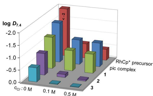
Figure 7. Logarithm of distribution coefficients ( \log D_{7.4} ) of the \text{RhCp}^* precursor, [\text{RhCp}^*(\text{pic})(\text{H}_2\text{O})]^+ and complexes 1–3 at pH 7.40 measured at various KCl concentrations (as indicated in the figure) \{C_{\text{compound}} = 200 \mu\text{M}; T = 25 \text{ }^\circ\text{C}, \text{ in } 20 \text{ mM phosphate buffer}\} . Log D_{7.4} values of the ligands measured at 0.1 M KCl content for comparison: 2-QA: -1.3(1) , 3-iQA: -1.41(4) and pic: <-2.0 [52], 6-Mepic: <-2.0 [52].
