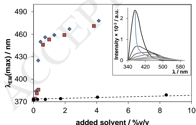
Fig. 3. Effect of solvent mixture composition on the emission maximum ( \lambda_{EM(max)} ) of ERL, dissolved in n -hexane with indicated amounts of methanol ( \blacklozenge ), ethanol ( \blacksquare ) or benzene ( \bullet ) added. The dotted line depicts the gradual increase of the \lambda_{EM(max)} ( R^2 = 0.997 , and the
