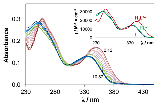
Fig. 1. UV–Vis absorbance spectra of AFA recorded at various pH values. Inset shows the individual molar absorbance spectra of the inhibitor in different protonation states denoted as H_2L^{2+} , HL^+ and L ( c_{lig} = 5 \mu M ; l = 2 \text{ cm} ; T = 25 \text{ }^\circ C ; I = 0.10 \text{ M (KCl)} ).
