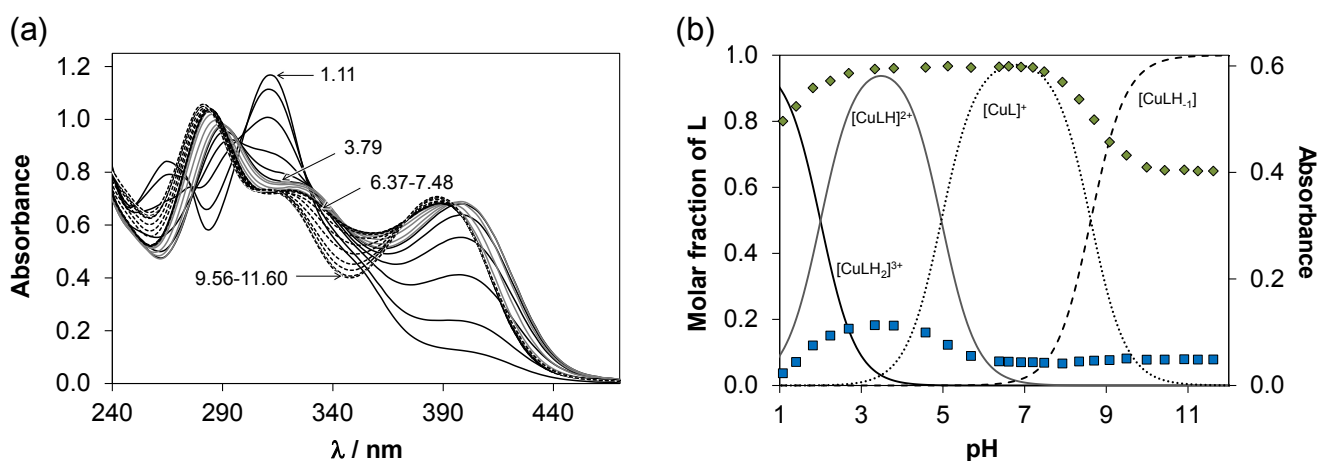
Figure 3. UV-vis spectra recorded for the Cu(II)- \text{HL}^1 (1:1) system at various pH values (a), and concentration distribution curves and measured absorbance values at 346 nm ( \blacklozenge ) and 440 nm ( \blacksquare ) for the same system (b). \{c_{\text{Cu(II)}} = c_{\text{lig}} = 121 \mu\text{M}; T = 298 \text{ K}; I = 0.10 \text{ M (KCl)}; l = 0.5 \text{ cm}\} .
