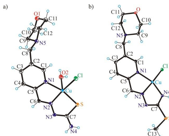
25 26 27 28 29 30 31 32 33 34 35 36 37 38 39 40 41 42 43 44 45 46 47 48 49 50 51 52 53 54 55 56 57 58 59 60 Figure 2. ORTEP views of (a) [Cu(L 1 )Cl(H 2 O)] ( 1 + ) and (b) [Cu(L 6 )Cl] ( 6 ).
