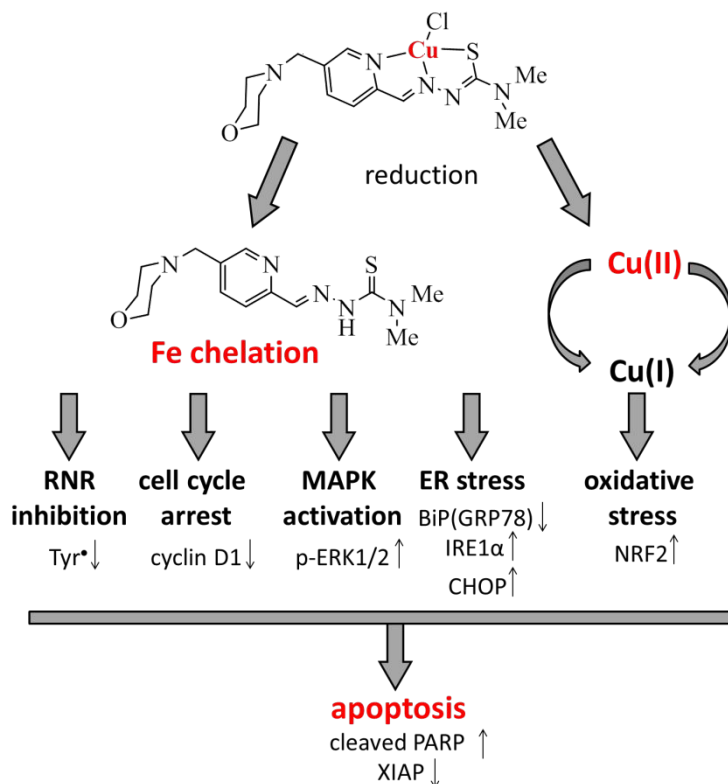
30 31 32 33 34 35 36 37 38 39 40 41 42 43 44 45 46 47 48 49 50 51 52 53 54 55 56 57 58 59 60 Figure 10. Proposed molecular mechanism of complex 2 .
