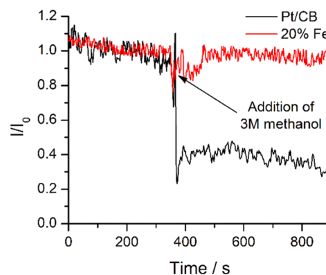
Figure 7. Alkaline (0.1 M KOH) chronoamperometric methanol tolerance ORR response at 0.51 V (vs RHE) of commercial Pt/CB catalyst and the 20 wt % Fe-containing composite deposited onto a glassy carbon electrode.
