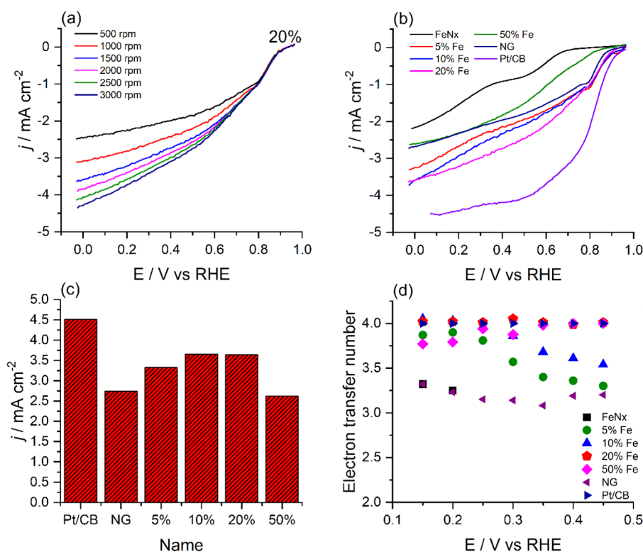
Figure 4. (a) LSV curves of the 20% iron-containing Fe x N/NG using rotating disk electrode at various rotation rates. (b) Voltammograms recorded at fixed 1500 rpm for the Fe x N/NG and Pt/CB composites on glassy carbon electrode (GCE). (c) Reduction current densities (at 0 V (vs RHE) and 1500 rpm) and (d) electron-transfer numbers were determined from LSV measurements. Voltammograms were recorded in alkaline conditions (0.1 M KOH) applying a scan rate of 10 mV s -1 .
