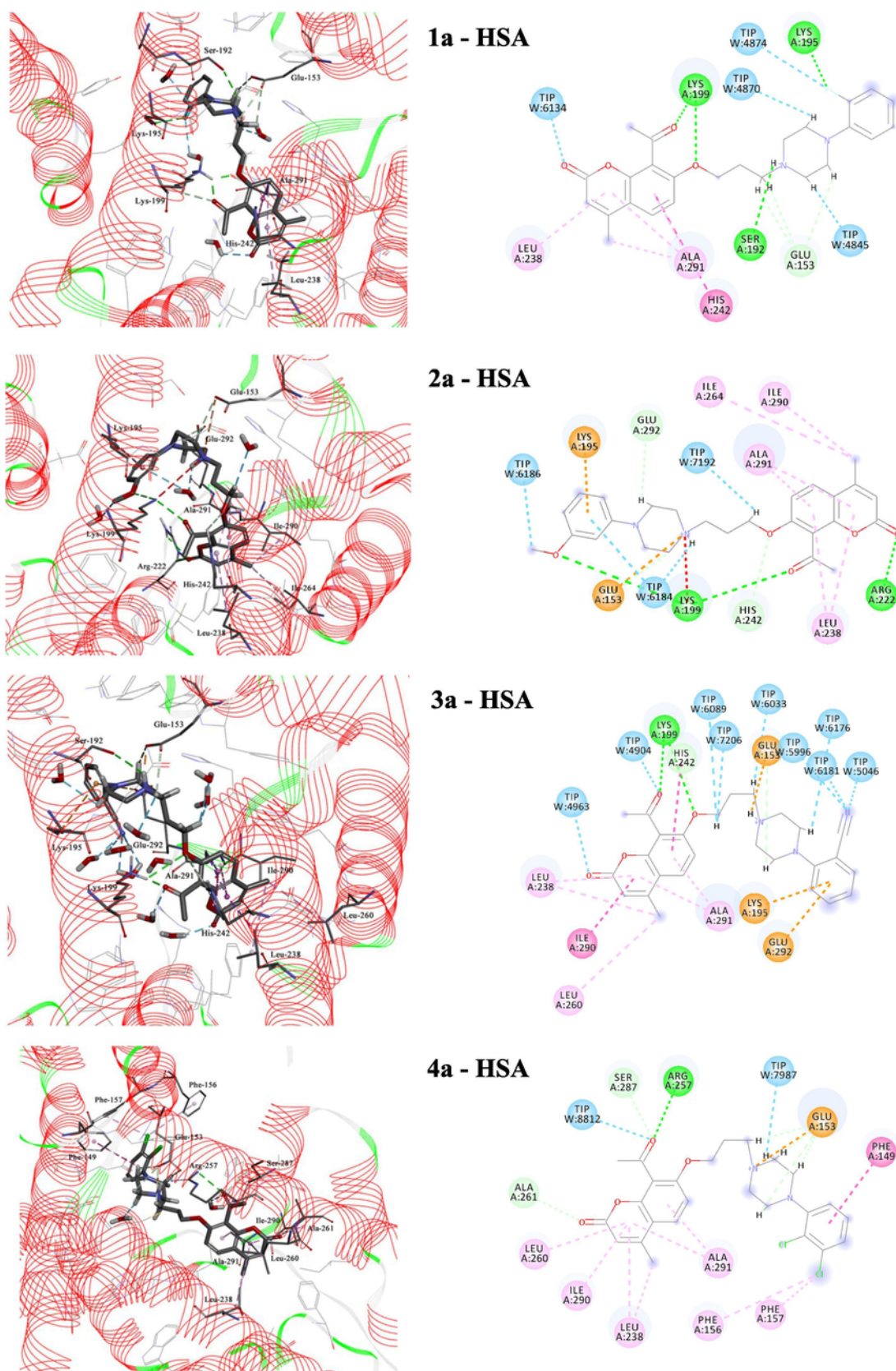
Fig. 9. Structures of the 1a HSA, 2a HSA, 3a HSA and 4a HSA complexes, and 2D view of all HSA residues interacting with the ligands resulting from MD simulations (residues involved in hydrogen bonding marked as green and cyan circles; in hydrophobic interactions marked as pink circle and electrostatic interactions marked as orange circle). (For interpretation of the references to colour in this figure legend, the reader is referred to the web version of this article.)
