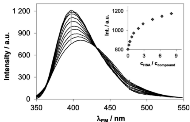
Fig. 7. Emission spectra of 3a upon addition of HSA. Inset shows the intensity changes at \lambda_{EM} = 410 nm. ( c_{comp} = 2.8 M; c_{HSA} = 0.23 M; \lambda_{EX} = 330 nm; t = 25 °C; pH = 7.40 (20 mM phosphate buffer); I = 0.10 M (KCl)). Spectra are corrected by the light scattering effect of HSA, see details in the Supplementary Materials, Fig S6.
