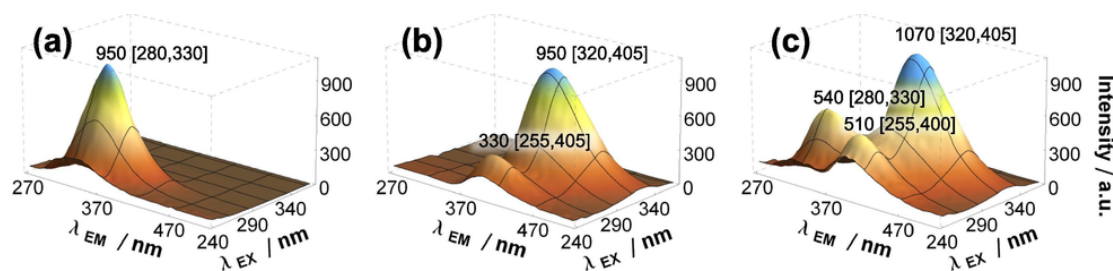
Fig. 6. Three-dimensional fluorescence spectra of HSA (a) compound 3a (b) and HSA-3a (1:11) system (c); peak intensities and wavelength coordinates (Intensity, I_{EM} , I_{EX} expressed in nm) are indicated in the figure ( c_{HSA} = 1 M; c_{comp} = 11 M; t = 25 °C; pH = 7.40 (20 mM phosphate buffer); I = 0.10 M (KCl)).
