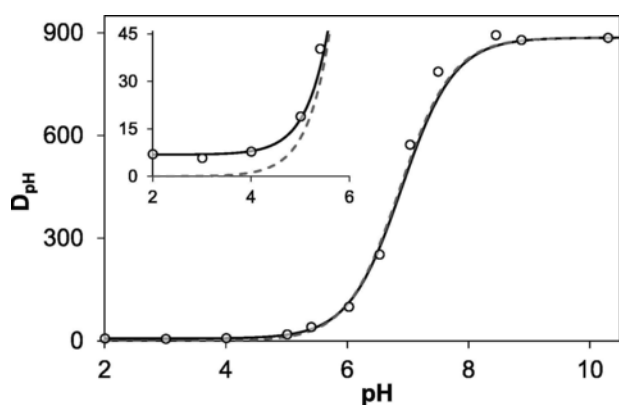
Fig. 3. Measured (○) and fitted distribution coefficients ( D_{\text{pH}} ) for 2a at different pH values. Fitted curves correspond to the model 1 where only the distribution of the neutral form is expected (dashed line), and to the model 2 where both L and HL + forms may distribute between the polar and non -polar phases (solid line). Inset shows the initial part of the functions in the pH range from 2.0 to 6.0. ( D_{\text{pH}} values were determined in n -octanol/water system at the indicated pH values by traditional shake flask method; see details in the Section 2.2.2).
