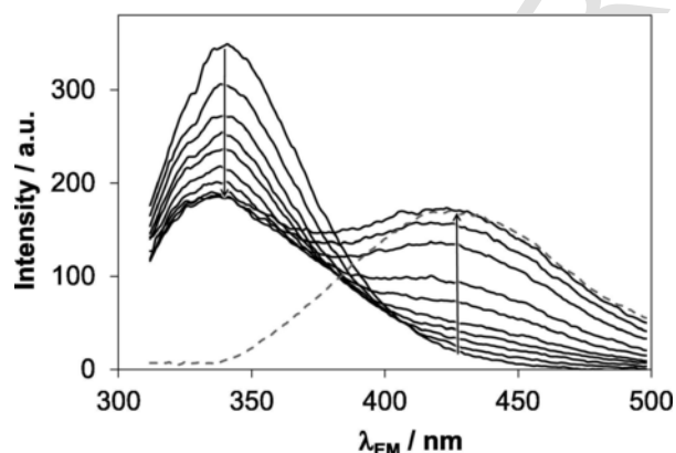
Fig. 4. Fluorescence emission spectra of HSA- 4a system. The grey dotted line shows the spectrum for 4a alone at 10 \mu\text{M} concentration. ( c_{\text{HSA}} = 1 \text{ M} ; c_{\text{comp}} = 0.10 \text{ M} ; \lambda_{\text{EX}} = 295 \text{ nm} ; t = 25^\circ\text{C} ; \text{pH} = 7.40 (20 mM phosphate buffer); I = 0.1 \text{ M (KCl)} ).
