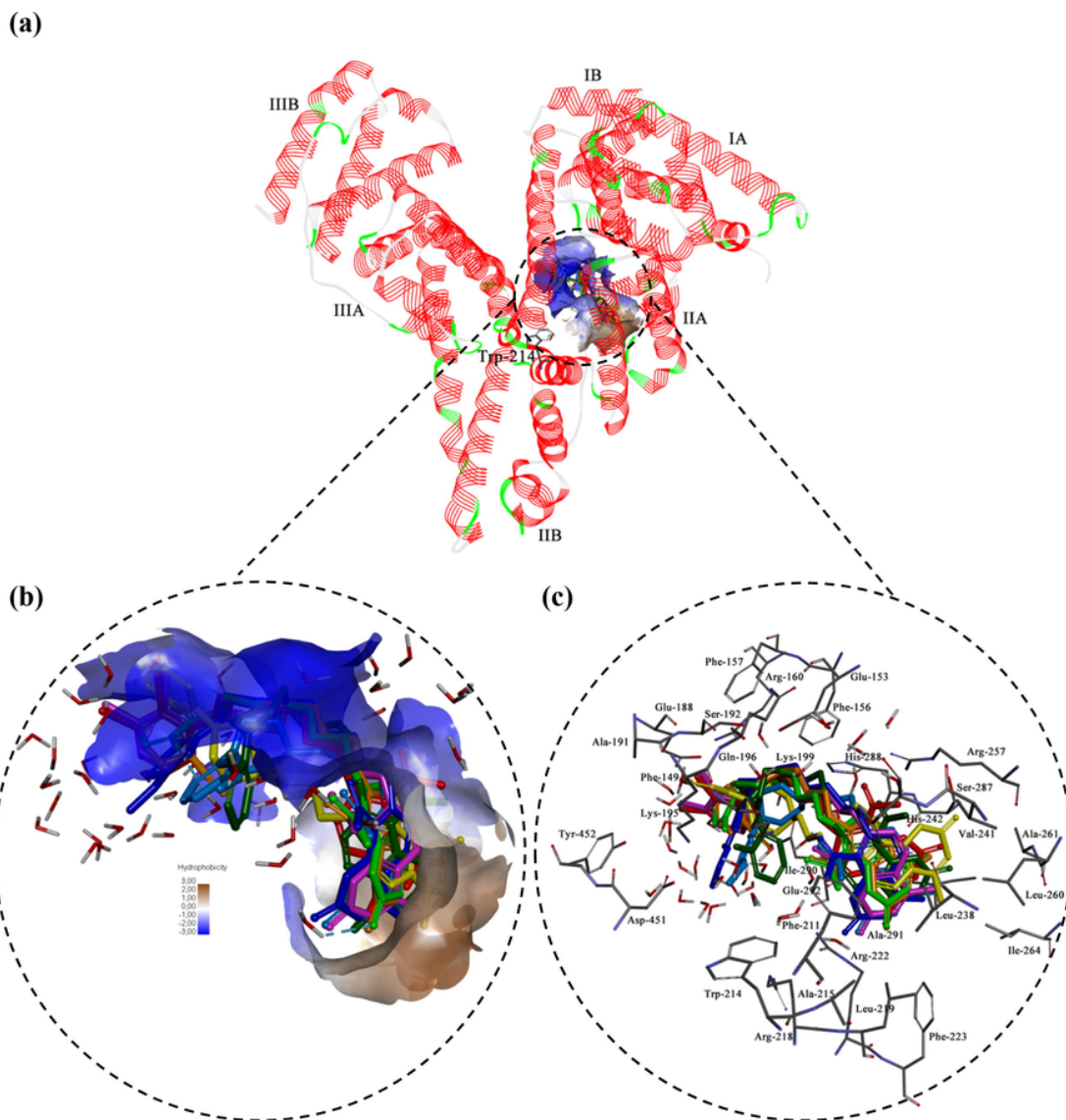
Fig. 8. View of coumarin derivatives in site 1 of HSA. (a) Structure of HSA showing the subdomains and binding sites of compounds 1a 4a and 1b 4b . Compounds around the binding pocket are shown as spheres. (b) The hydrophobic and hydrophilic amino acid residues surrounding the ligands. Surface hydrophobicity was depicted by the shaded colors: brown the hydrophobic and blue lipophilic regions. (c) Superposition of compounds: 1a (green), 2a (blue), 3a (orange), 4a (red), 1b (dark green), 2b (dark blue), 3b (yellow) and 4b (pink). (For interpretation of the references to colour in this figure legend, the reader is referred to the web version of this article.)
