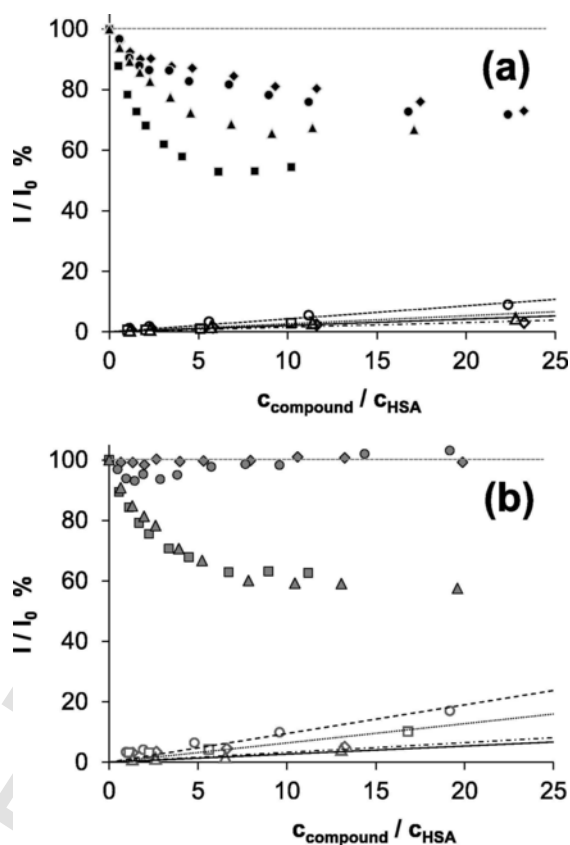
Fig. 5. Measured quenching of the Trp fluorescence emission intensity of HSA as I/I_0 (%) by the addition of the propyloxy derivatives (a): 1a (○), 2a (□); 3a (△); 4a (◇), and butyloxy derivatives (b): 1b (○), 2b (□); 3b (△); 4b (◇). Empty symbols correspond to the relative emission of the compounds alone. ( c_{\text{HSA}} = 1 \text{ M} ; \lambda_{\text{EX}} = 295 \text{ nm} ; \lambda_{\text{EM}} = 340 \text{ nm} ; t = 25^\circ\text{C} ; \text{pH} = 7.40 (20 mM phosphate buffer); I = 0.10 \text{ M (KCl)} ).
