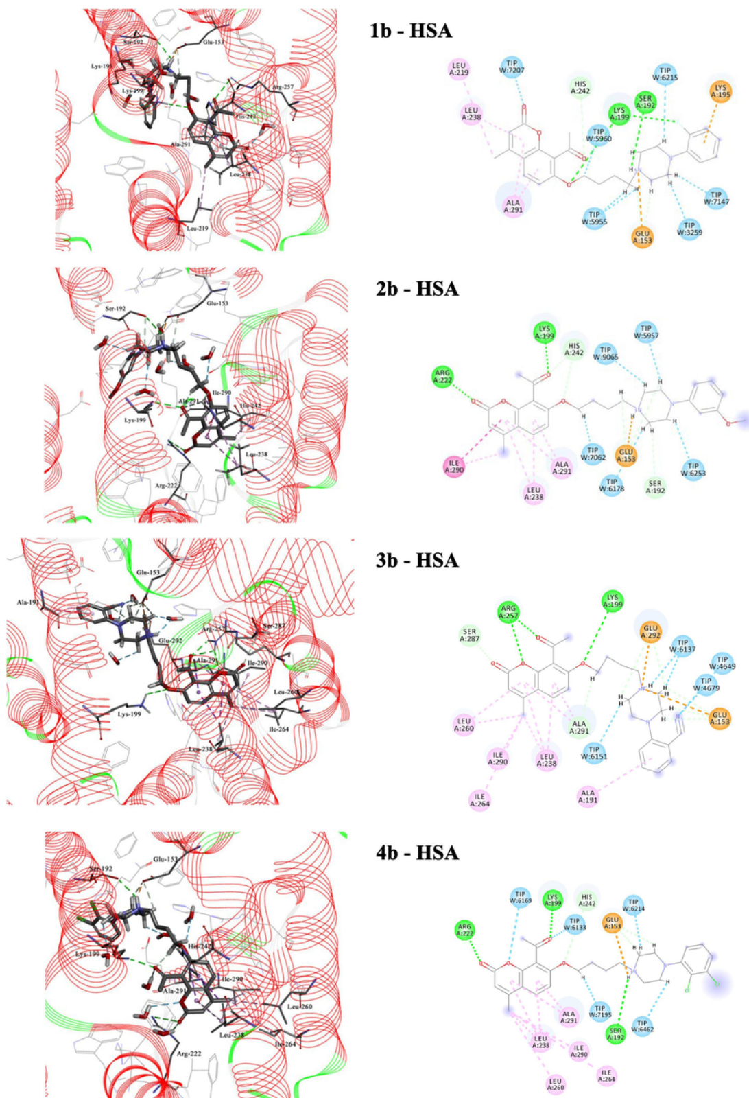
Fig. 10. Structures of the 1b HSA, 2b HSA, 3b HSA and 4b HSA complexes, and 2D view of all HSA residues interacting with the ligands resulting from MD simulations (residues involved in hydrogen bonding marked as green and cyan circles; in hydrophobic interactions marked as pink circle and electrostatic interactions marked as orange circle). (For interpretation of the references to colour in this figure legend, the reader is referred to the web version of this article.)
