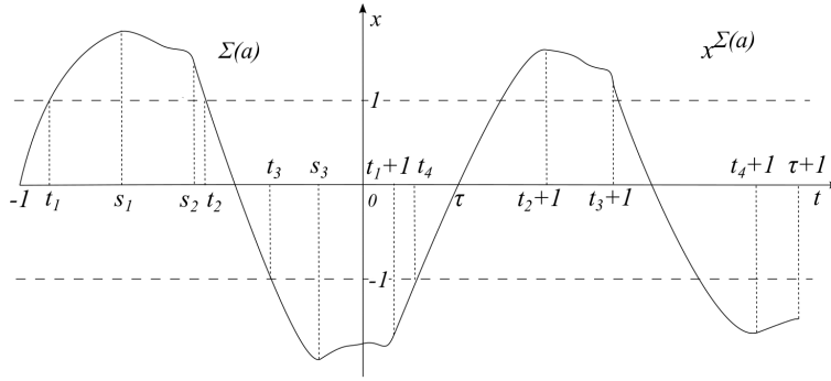
Figure 4.2: The plot of an element of \Sigma(U^1) and of the corresponding solution.
