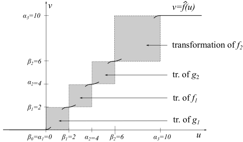
Figure 6.2: The plot of \hat{f} in our example. On the interval [0, 10] , the graph of \hat{f} lies in the gray squares.
