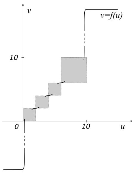
Figure 6.3: The plot of f in our example.
