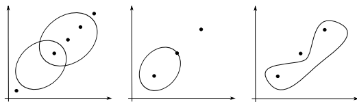
Figure 1.1: Three examples excluded by Mallet-Paret and Sell. Here we show the images of periodic orbits and equilibria under \pi_2 .
