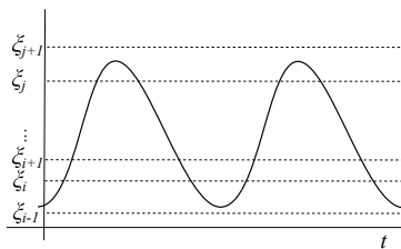
Figure 2.2: An [i, j] periodic function.
