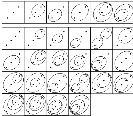
Figure 1.2: Possible configurations for three or four unstable equilibria: The images of the large-amplitude periodic orbits and the unstable equilibria under \pi_2 .
