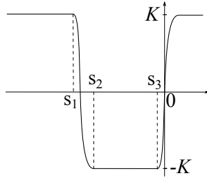
Figure 4.1: The plot of h(a) .
