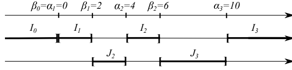
Figure 6.1: The partition of the real line in our example.
