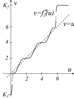
Figure 5.2: The plot of f_3^* . Observe that f_3 has to be modified for u < \eta and for u > 6 - \eta .
