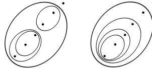
Figure 2.3: Configurations corresponding to the expressions ((1(23))(45))6 and ((((12)3)4)5)6 .
