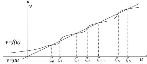
Figure 2.1: A nonlinearity f giving N unstable and N + 1 stable equilibria.
