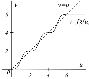
Figure 5.1: The plot of f_3 .
