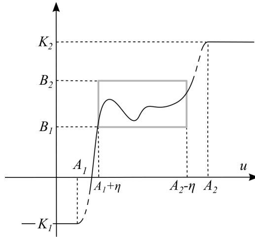
Figure 4.3: The plot of f in Corollary 4.10.
