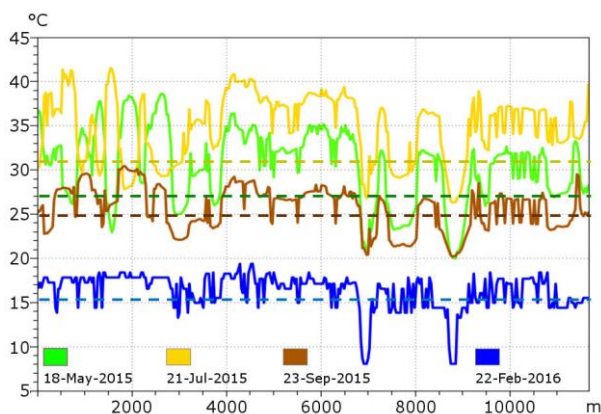
Fig. 6 Temporal patterns of LST (the dashed line represents the mean temperature of the rural areas)
