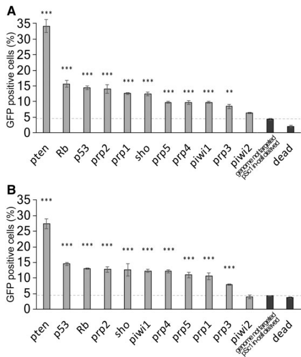
Figure 3. The efficiency of different spacers to mediate targeted integration when used with self-cleaving GFP-plasmids in N2a cells. The efficiencies of different spacers in targeted integration using the pSc1 (A) or pSc2 (B) self-cleaving GFP-plasmid are assessed. The percentages of the cells harbouring stably integrated GFP-cassette were measured for 11 different spacers (pten, Rb, p53, prp1-5, sho, piwi1-2) targeting seven genes ( Pten , Rbl2 , Tp53 , Prnp , Sprn , Piwil4 , Piwil2 ) as indicated by the light grey bars, when co-transfecting with either the circular pSc1 (A) or pSc2 (B) self-cleaving GFP-plasmids. To measure the random integration background of the self-cleaving plasmids, they were co-transfected with a vector expressing active SpCas9 and the corresponding TL gRNA; thus, the genome is not targeted, but the self-cleaving plasmids are linearized (genome not targeted, Sc1 in-cell cleaved; A and B, indicated by the dashed lines). Bars show the means \pm S.D. of percentages measured in n = 3 independent transfections, which were normalized to the transfection efficiency (% GFP positive cells measured on 2nd day after transfection: ranging between 94 and 98%). Values obtained are compared to the control where the linearized self-cleaving GFP-plasmid (genome not targeted, pSc1 in-cell cleaved) was used. *** P < 0.001 .
