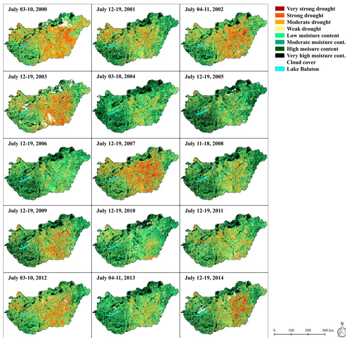
Fig. 5 Geographic distribution of drought areas according to NDWI in July
